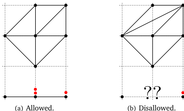
Figure 4: Left: An example of an allowed vertical reduction of a toric diagram \Gamma , leading to a resolved A_1 singularity \widehat{Y} , pictured by the 1d toric diagram at the bottom. The vertical lines in the middle of \Gamma are mapped to a single exceptional curve D_1^{\widehat{Y}} \cong \mathbb{P}^1 \subset \widehat{Y} wrapped by two D6-branes. The vertical line on the right of \Gamma is mapped to a single D6-brane along the non-compact divisor D_2^{\widehat{Y}} \cong \mathbb{C} \subset \widehat{Y} . Right: An example of a triangulation without an allowed vertical reduction, because there is an edge with \Delta v = (2, 1, 0) .
