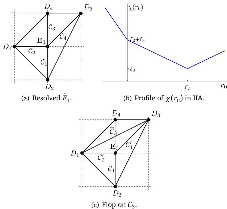
Figure 8: The resolved \tilde{E}_1 singularity and its vertical reduction. By flopping C_3 and sending \text{vol}(\tilde{C}_3) to infinity (that is, \xi_3 \rightarrow -\infty ), one obtains the isolated E_0 theory.
