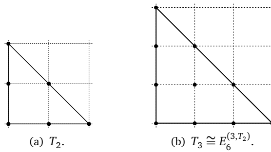
Figure 27: The T_2 “rank-zero” toric geometry, and the T_3 toric geometry. They have 3 and 30 allowed vertical resolutions, respectively.
