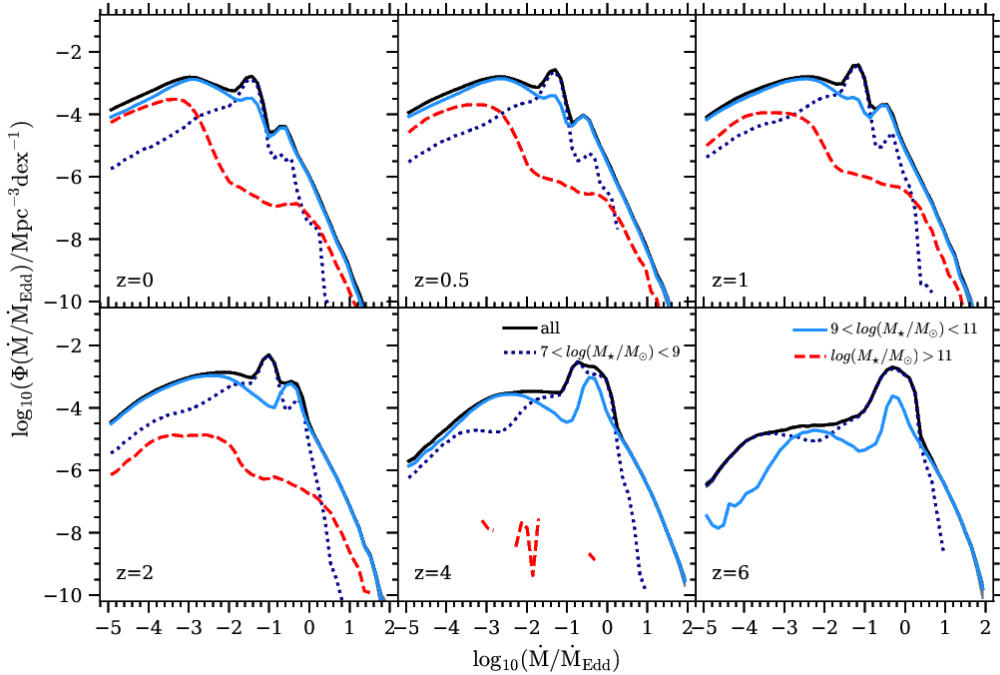
Figure 7. The distribution of Eddington ratio in terms of mass accretion rate, \dot{M}/\dot{M}_{\text{Edd}} , evolving with redshift. Shown are all objects with stellar mass, M_{\star} > 10^7 M_{\odot} (black solid line), objects with stellar mass 10^7 M_{\odot} < M_{\star} < 10^9 M_{\odot} (dark blue dotted line), objects with stellar mass 10^9 M_{\odot} < M_{\star} < 10^{11} M_{\odot} (light blue solid line) and objects with stellar mass M_{\star} > 10^{11} M_{\odot} (red dashed line).
