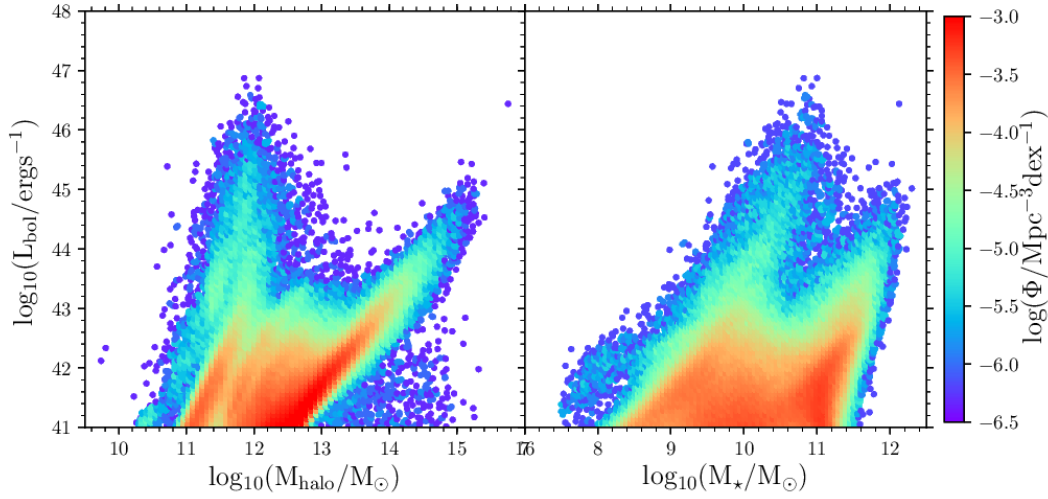
Figure 12. Left panel: a scatter plot of AGN bolometric luminosity versus halo mass at z = 0 . The points are coloured by the density of objects in this plane, where red indicates a high density of objects while blue indicates a low density of objects. Right panel: as in the left panel but showing bolometric luminosity versus stellar mass.
