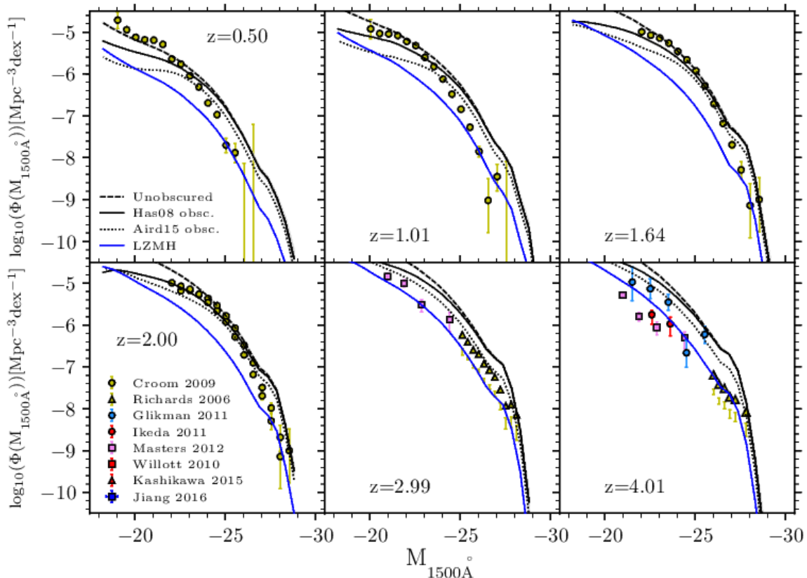
Figure 19. The predicted rest-frame 1500\text{\AA} luminosity function compared to observations which have been converted to 1500\text{\AA} . The dashed black line is the prediction without accounting for absorption effects, the solid black line is the prediction with the Hasinger (2008) visible fraction, the dotted black line is with the Aird et al. (2015) visible fraction and the blue line is with my observationally determined LZMH visible fraction. The observations are from SDSS DR3 Richards et al. (2006) (yellow triangles), 2SLAQ+SDSS Croom et al. (2009) (yellow circles), CFHQS+SDSS Willott et al. (2010) (red squares), NDWFS+DLS Glikman et al. (2011) (blue circles), the COSMOS field Ikeda et al. (2011) (red circles), Masters et al. (2012) (purple squares), Subaru Kashikawa et al. (2015) (red triangles) and SDSS Stripe 82 Jiang et al. (2016) (blue squares).
