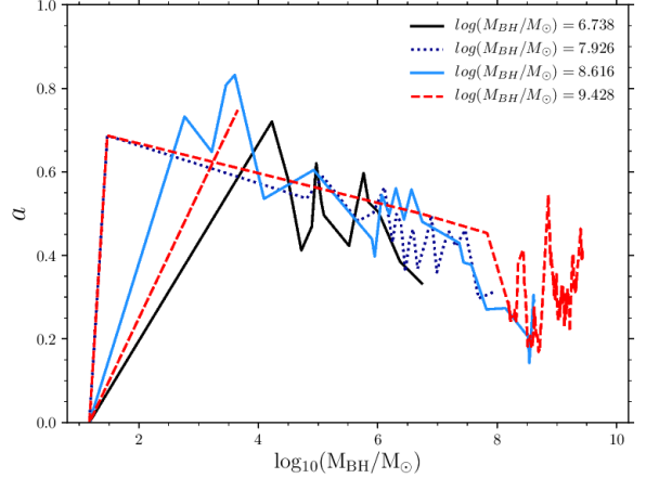
Figure 11. The evolution of four different mass SMBHs through the spin versus mass plane. The final SMBH masses at z = 0 are the same as plotted in Figure 10.
