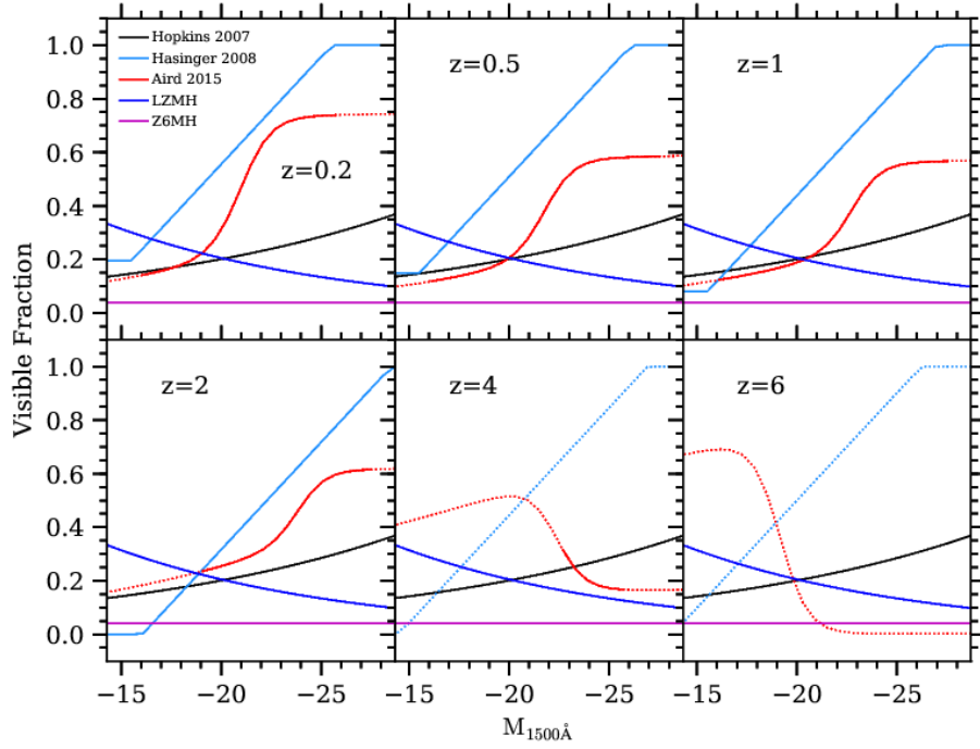
Figure C1. Comparing the visible fractions for rest-frame 1500Å for different obscuration models. Shown are Hopkins et al. (2007) (black), Hasinger (2008) (light blue), Aird et al. (2015) (red), the LZMH model (dark blue) and the Z6MH model (purple). The solid lines for the observational visible fractions indicate the ranges where there is observational data, while the dotted lines indicate ranges where a functional form has been extrapolated.
