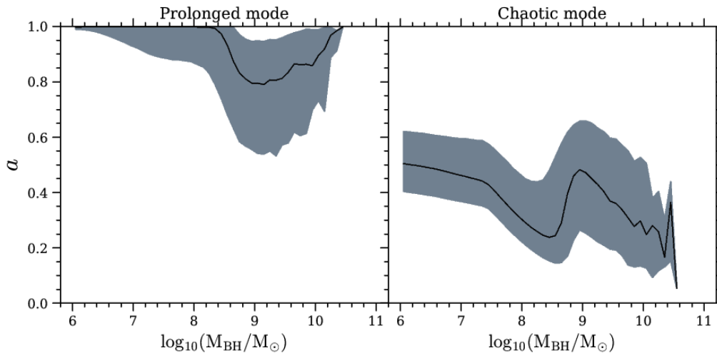
Figure 8. The predicted SMBH spin distributions at z = 0 for prolonged (left panel) and chaotic (right panel) accretion modes. The line represents the median value of the magnitude of the spin for that SMBH mass, and the shading represents the 10-90 percentile range of the distribution.
