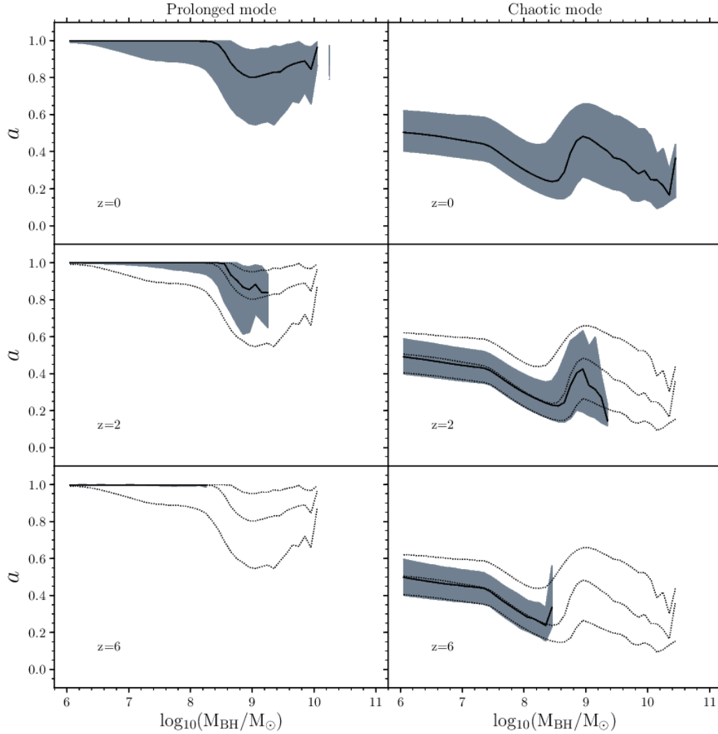
Figure 9. The predicted evolution of the SMBH spin distribution for prolonged mode (left panels) and chaotic mode (right panels). Results are shown for z = 0, 2, 6 . The lines and shading have the same meaning as in the previous figure, with the dotted line representing the median and percentiles for that accretion mode at z = 0 .
