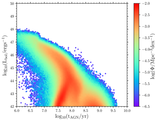
Figure 13. As in Figure 12 but showing the dependence of AGN bolometric luminosity on the duration of the AGN episode, for starburst mode fuelled AGN only.
