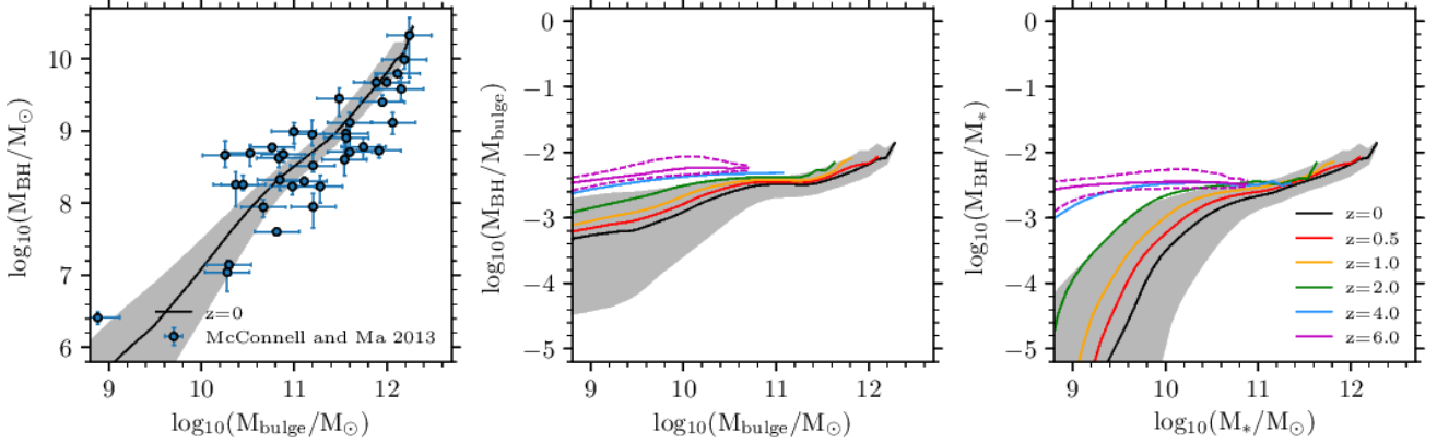
Figure 5. Left panel: the predicted SMBH mass versus bulge stellar mass relation at z = 0 compared to observational data from McConnell & Ma (2013). The line represents the median of the predicted SMBH mass in bins of bulge mass and the shading denotes the 10-90 percentiles of the predicted distribution. Middle panel: the evolution of the median of the ratio of SMBH mass to bulge mass versus bulge mass relation with redshift for z = 0, 0.5, 1, 2, 4, 6 . As in the left panel, the grey shaded band is the 10-90 percentiles of the distribution for z = 0 and the purple dashed lines are the 10-90 percentiles of the distribution for z = 6 . Right panel: the evolution of the median of the ratio of SMBH mass to galaxy stellar mass versus galaxy stellar mass relation, with the lines representing the same redshifts as the middle panel as indicated by the legend.
