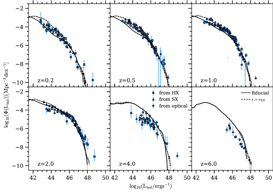
Figure E5. Exploring the effect of changing the accretion efficiency \epsilon : the model with \epsilon = \epsilon_{TD} as the accretion efficiency for all \dot{m} regimes (black dashed) and the fiducial model (black solid).
