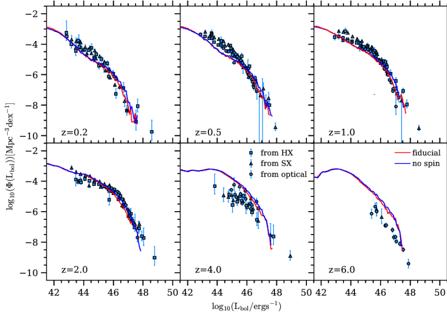
Figure E4. Exploring the effect of turning off the SMBH spinup evolution: the model with chaotic mode accretion spinup and merger spinup (red) and the model with no accretion nor merger spinup with a thin disc accretion efficiency, \epsilon_{TD} = 0.1 (blue).
