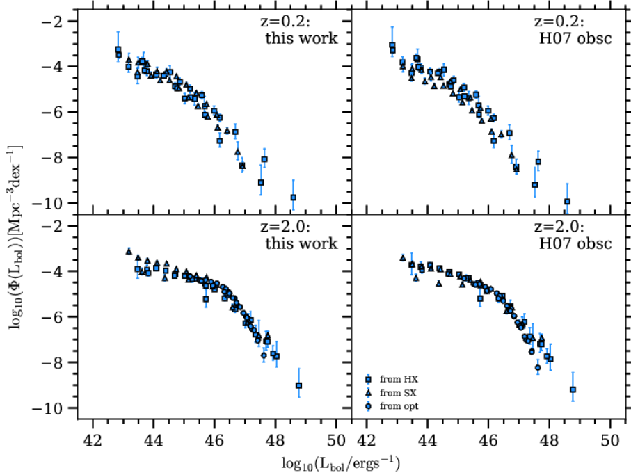
Figure C4. Comparing the effect of using different obscuration models on the constructed bolometric luminosity functions. The left panels are obtained using the obscuration model presented in this work, while the right panels use the obscuration model of Hopkins et al. (2007) . The upper panels are for z = 0.2 and the lower panels are for z = 2 .
