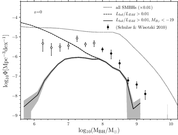
Figure 4. The active black hole mass function (solid line) at z = 0 , compared to observational estimates from Schulze & Wisotzki (2010). We show predictions where active SMBHs are defined as AGN brighter than a threshold Eddington ratio ( L_{\text{bol}}/L_{\text{Edd}} > 0.01 ), using the LZMH visible fraction (c.f. Section 3.3) (dashed line), and predictions also brighter than a threshold AGN absolute magnitude ( M_{\text{BJ}} < -19 ) (solid line). This is for appropriate comparison with the active black hole mass function in Schulze & Wisotzki (2010), where the open circles are the data points that suffer from incompleteness, while the filled circles are the data points that do not. We also show the total black hole mass function (dotted line) with the number density divided by 100, for comparison.
