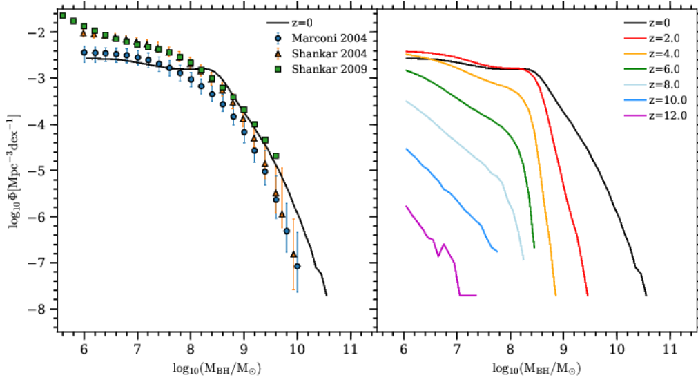
Figure 3. The black hole mass function. Left panel: the predicted black hole mass function at z = 0 compared to observational estimates by Marconi et al. (2004); Shankar et al. (2004, 2009). Right panel: the evolution of the black hole mass function over the range 0 < z < 12 .
