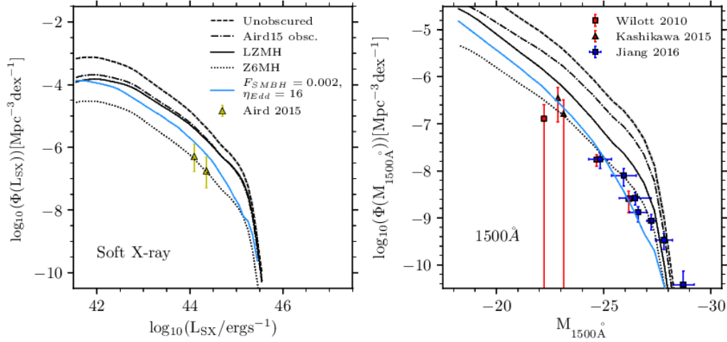
Figure 20. The rest-frame soft X-ray luminosity function (left panel) and the rest-frame 1500Å luminosity function (right panel), both at z = 6 . We show predictions without obscuration (dashed black), with the Aird et al. (2015) visible fraction (dot-dash), with the ‘low z modified Hopkins’ (LZMH) visible fraction with the standard model (black solid), with the ‘ z = 6 modified Hopkins’ (Z6MH) visible fraction (black dotted) and with the ‘low z modified Hopkins’ visible fraction with the different parameters (blue solid). The observations for the soft X-ray band are from Aird et al. (2015) (yellow triangles), and for 1500Å are from Willott et al. (2010) (red squares), Kashikawa et al. (2015) (red triangles) and Jiang et al. (2016) (blue squares).
