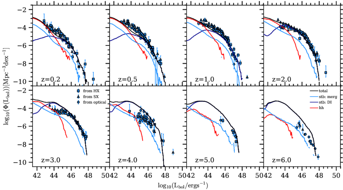
Figure 15. The AGN bolometric luminosity function as Figure 14, but split by the fuelling mode: starbursts triggered by mergers (light blue), starbursts triggered by disc instabilities (dark blue), hot halo mode (red).
