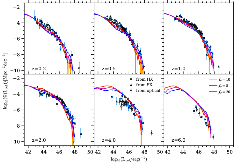
Figure E1. Exploring the effect on the AGN bolometric luminosity function of varying the parameter f_q . Shown are f_q = 5 (blue), f_q = 10 (purple, the fiducial model) and f_q = 20 (red). The shading shows the Poisson errors of the distribution.
