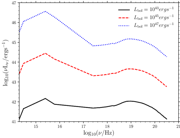
Figure 2. The Marconi et al. (2004) SED used for calculating luminosities in different wavebands in this work. Shown is the SED for L_{\text{bol}} = 10^{43} \text{ergs}^{-1} (black solid line), L_{\text{bol}} = 10^{45} \text{ergs}^{-1} (red dashed line) and for L_{\text{bol}} = 10^{47} \text{ergs}^{-1} (blue dotted line).
