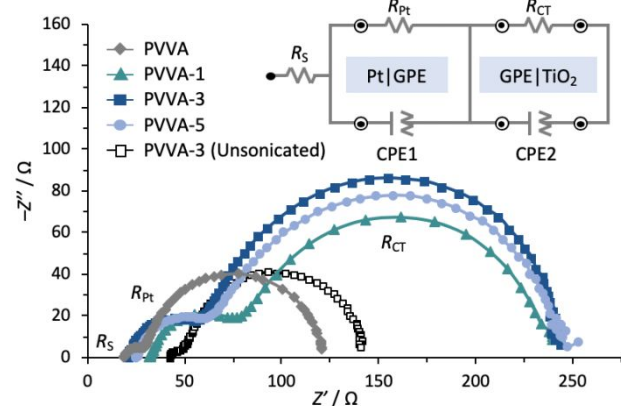
Figure 4. Electrochemical impedance data collected for GPE-based DSSCs show that sonochemically processed \text{Co}_3\text{O}_4 additives confer higher resistance ( R_{CT} ) towards charge recombination events (i.e., of \text{I}_3^- ) in GPEs, thus enabling fast N719 dye regeneration for enhanced DSSC performance. Inset: An equivalent circuit model has been fitted to the EIS data.
