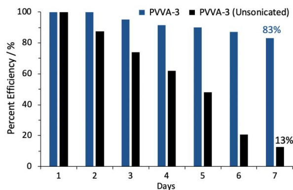
Figure 5. Photovoltaic performance stability of DSSCs employing \text{Co}_3\text{O}_4 -modified GPEs, plotted as percent efficiency over time. The sonochemically enhanced DSSC consisting of the GPE PVVA-3 retains 83% of its initial efficiency over the course of seven days, whereas the untreated cell is found to experience an 87% efficiency loss in the same period.
