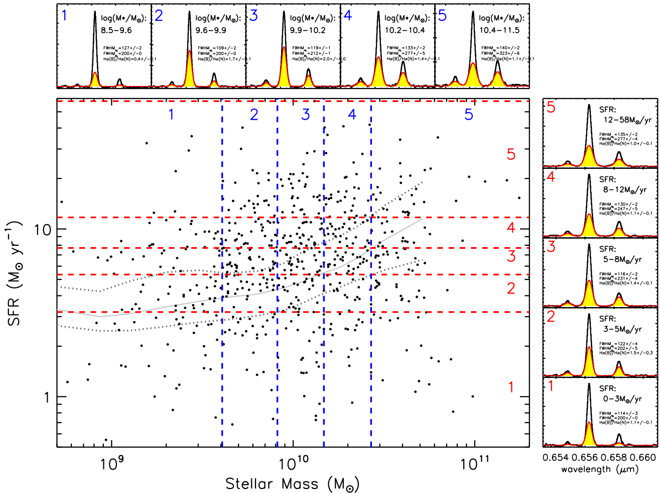
Figure 5. Stacked spectra for the galaxies in our sample as a function of stellar mass and SFR. The main panel shows the stellar masses and SFRs for the sample. We bin the sample in to 5 bins of stellar mass and SFR (labelled 1–5 in each case). Each bin contains the same number of galaxies, and are shown by the dashed lines. The panels across the top and right-hand side of the figure show the stacked spectra for each bin, including the underlying broad-line emission. These plots demonstrate that the broad, underlying emission increases in FWHM with increasing stellar mass and SFR.
