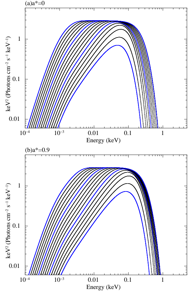
Figure 4. The emergent spectra for a 10^7 M_\odot black hole with different \dot{m} from \log \dot{m} = 0 to 2 with \Delta \dot{m} = 0.2 . Distance and inclination are set to be 100 Mpc and 0^\circ , respectively. Colours are the same as Fig. 3
