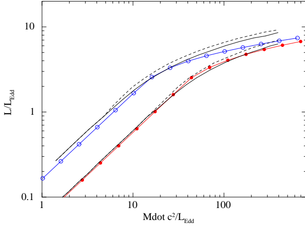
Figure 6. Eddington ratio as a function of \dot{M} c^2/L_{\text{Edd}} based on AGNSLIM. Same as Fig. 5, solid lines and dashed lines are theoretical predictions by Sądowski (2011) in Fig. 4.11, with \alpha = 0.01 and 0.1 . Case of black hole spin of a^* = 0 and 0.9 are shown with red filled circles and blue open circles, respectively.
