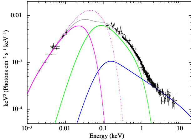
Figure 10. Same as Fig. 9 but with the best fit AGNSLIM model for a black hole mass 8 \times 10^6 M_\odot and a^* = 0 (grey), showing the outer blackbody disc (magenta), warm comptonised disc-corona (green) and hot inner disc-corona (blue). The dashed magenta line shows the same slim disc model but with pure blackbody emission at all radii.
