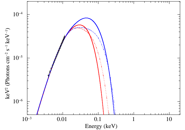
Figure 11. The best fit AGNSLIM model overlaid on the redshift corrected NIR spectrum of PSO J006 + 35. Solid lines and dotted lines correspond to i = 0^\circ and 60^\circ , respectively. Spin parameter a^* is assumed to be 0 (red) and 0.9 (blue).
