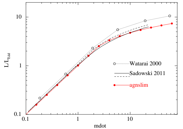
Figure 5. Eddington ratio as a function of \dot{m} based on AGNSLIM. Data points of AGNSLIM, Fig.3 of Watarai et al. (2000) are shown with filled red circles and open black circles, respectively. A solid line and a dashed line is theoretical prediction by Sądowski (2011) in Fig. 4.11, with \alpha = 0.01 and 0.1.
