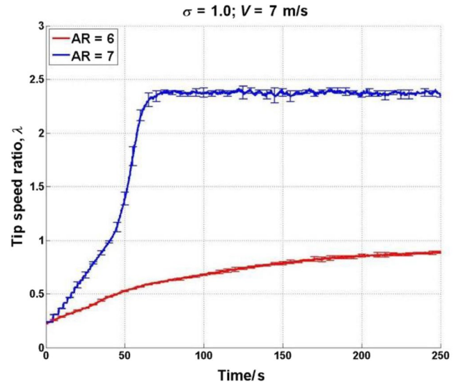
FIGURE 20 Self-starting time-varying results for turbine with different blade aspect ratios at \sigma = 1.0
