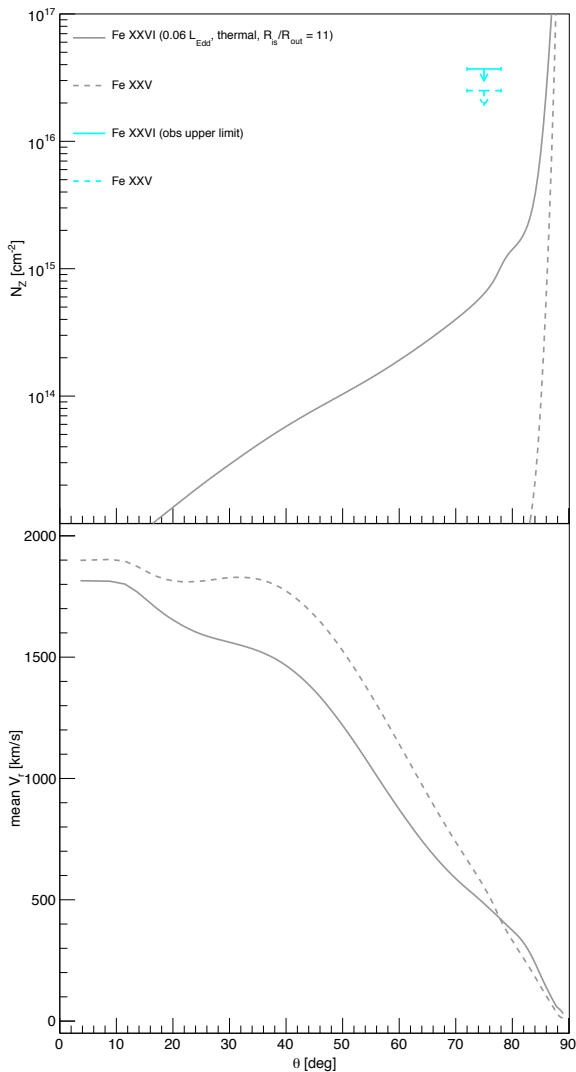
Figure 10. The angular dependence of column densities Fe XXVI (black solid line), Fe XXV (black dashed line) and those of column weighted velocities (bottom) of hard state. The cyan colars show the observational upper limit calculated from Miller et al. (2012)
