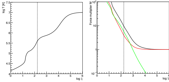
Figure 2. a) Thermal equilibrium curve of \log \xi vs \log T . b): Force multiplier of continuum process (bound-free plus scattering, red), line (green) and total (black) at the thermal equilibrium state. The vertical dashed line shows \xi_{H,\min} = 1.7 \times 10^2 which is the ionisation parameter of disc surface.
