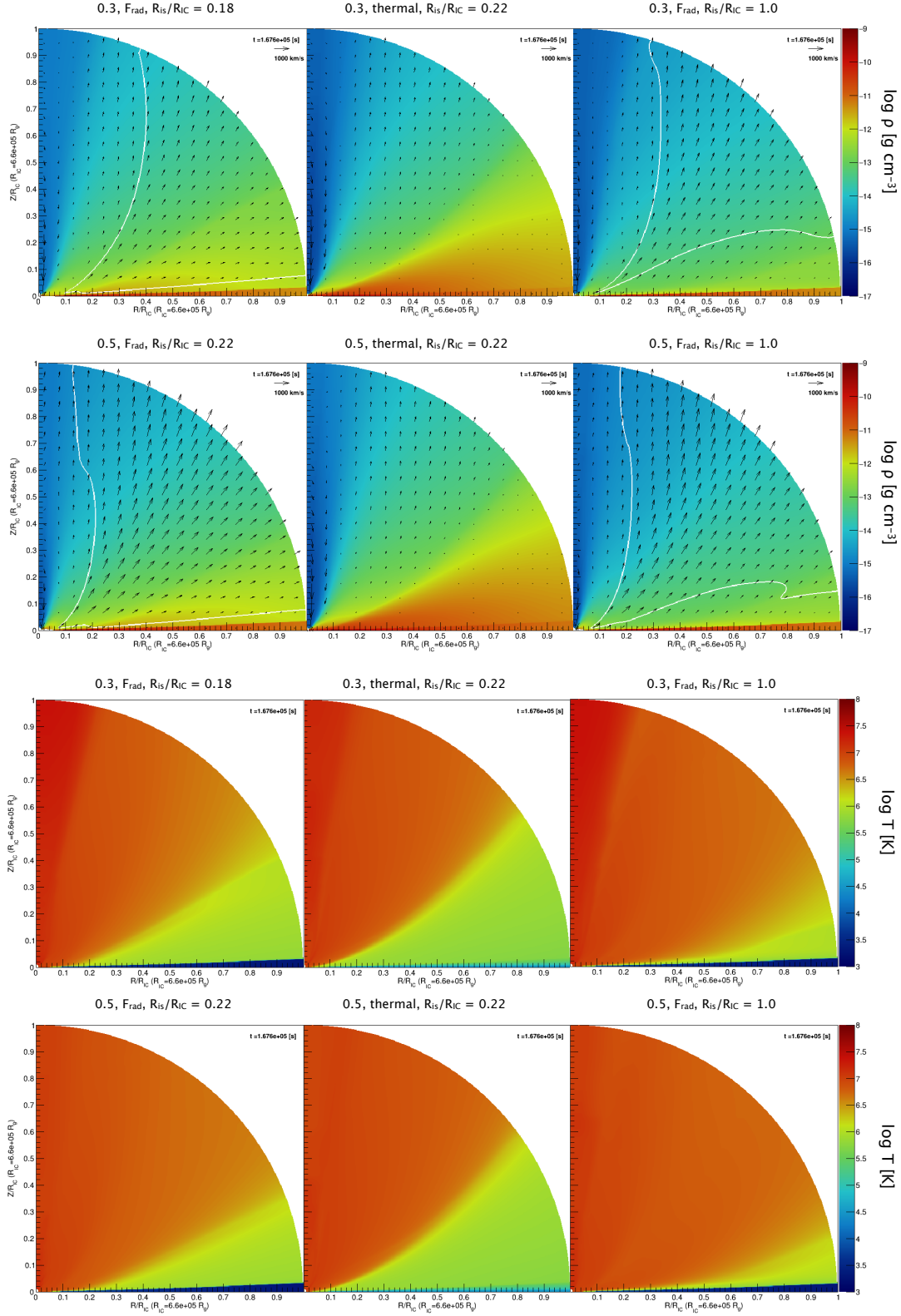
Figure B1. The density (top) and temperature (bottom) structures of final state of each simulation. Solid white lines show the Mach 1 surface of the outflow ( v_R/c_s = v_R/\sqrt{\gamma kT/(\mu m_p)} = 1 ).
