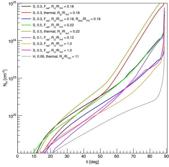
Figure B4. hydrogen column density of all simulations in Tab. 1
