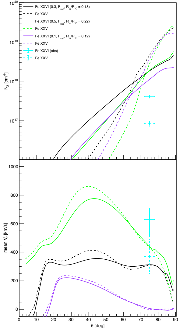
Figure 7. As in Fig.4 but for L/L_{\text{Edd}} = 0.1 (violet), 0.3 (black), 0.5 (green)
