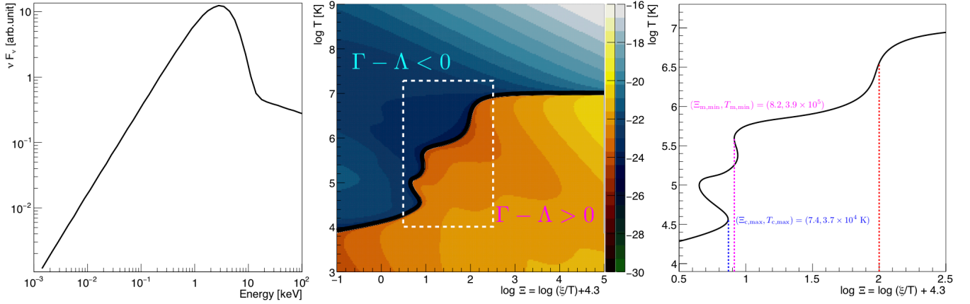
Figure 1. a) The energy flux of H 1743-322 which consists of a disc-blackbody plus Comptonised power-law (DISKBB+DISKBB*SIMPLE in XSPEC). b) The heating and cooling function ( \Gamma - \Lambda ). The black curve shows the thermal equilibrium ( \Gamma - \Lambda = 0 ), the right colour bar shows the absolute logarithm value of heating minus cooling function ( \log|\Gamma - \Lambda| ). The Compton temperature of this spectrum is T_{IC} = 1.0 \times 10^7 K. c) The zooming figure of b) surrounding by white dashed line. The vertical lines show the instability points. Red vertical lines is \Xi_{n,\min} = 100 .
