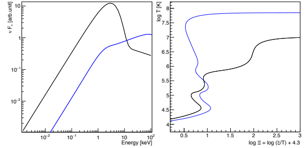
Figure 9. a) Spectra of soft state (black) and hard state (blue). b) The thermal equilibrium curves. colours correspond to input spectra of a) .
