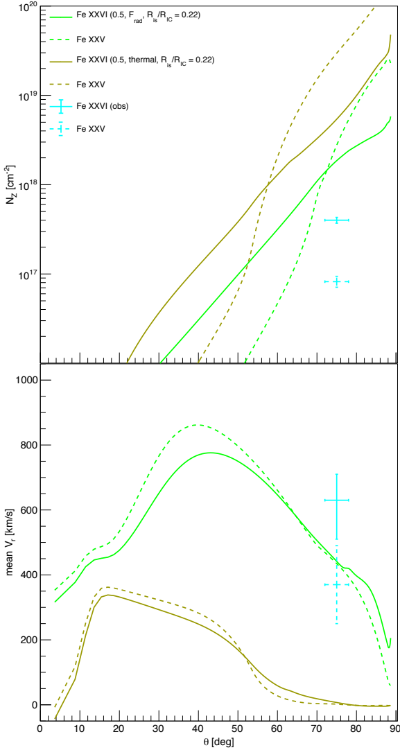
Figure 6. As Fig.4 but for L = 0.5L_{\text{Edd}} .
