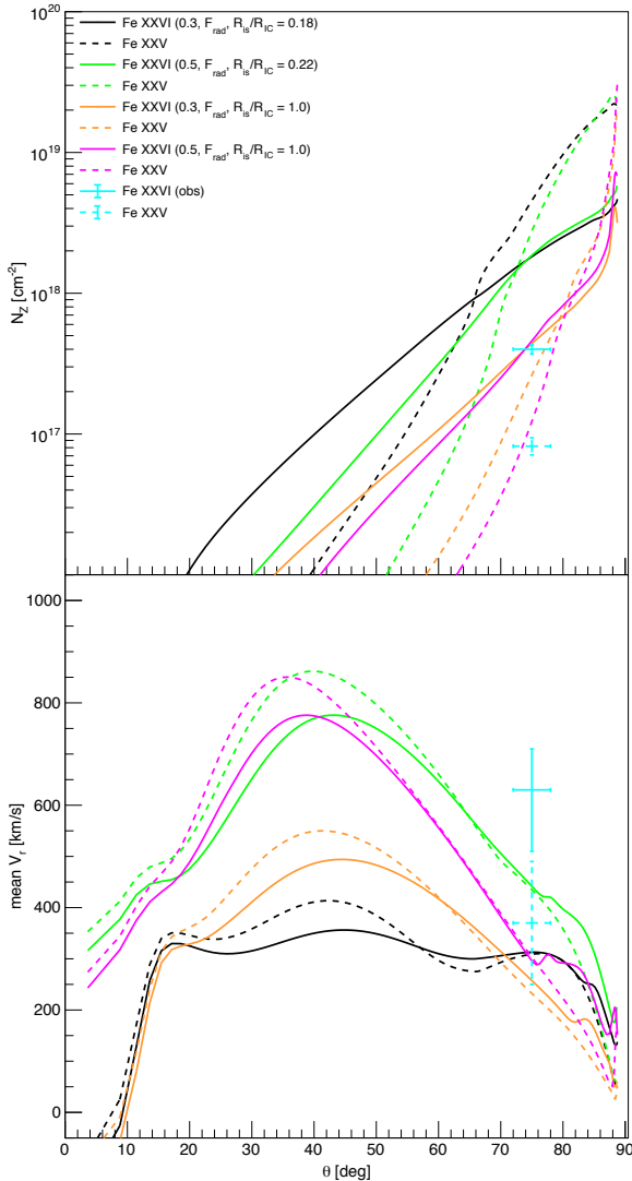
Figure 8. As in Fig.4 but for L/L_{\text{Edd}} = 0.3 , R_{\text{IS}}/R_{\text{IC}} = 0.18 (black), L/L_{\text{Edd}} = 0.5 , R_{\text{IS}}/R_{\text{IC}} = 0.22 (green), L/L_{\text{Edd}} = 0.3 , R_{\text{IS}}/R_{\text{IC}} = 1.0 (orange), and L/L_{\text{Edd}} = 0.5 , R_{\text{IS}}/R_{\text{IC}} = 1.0 (magenta).
