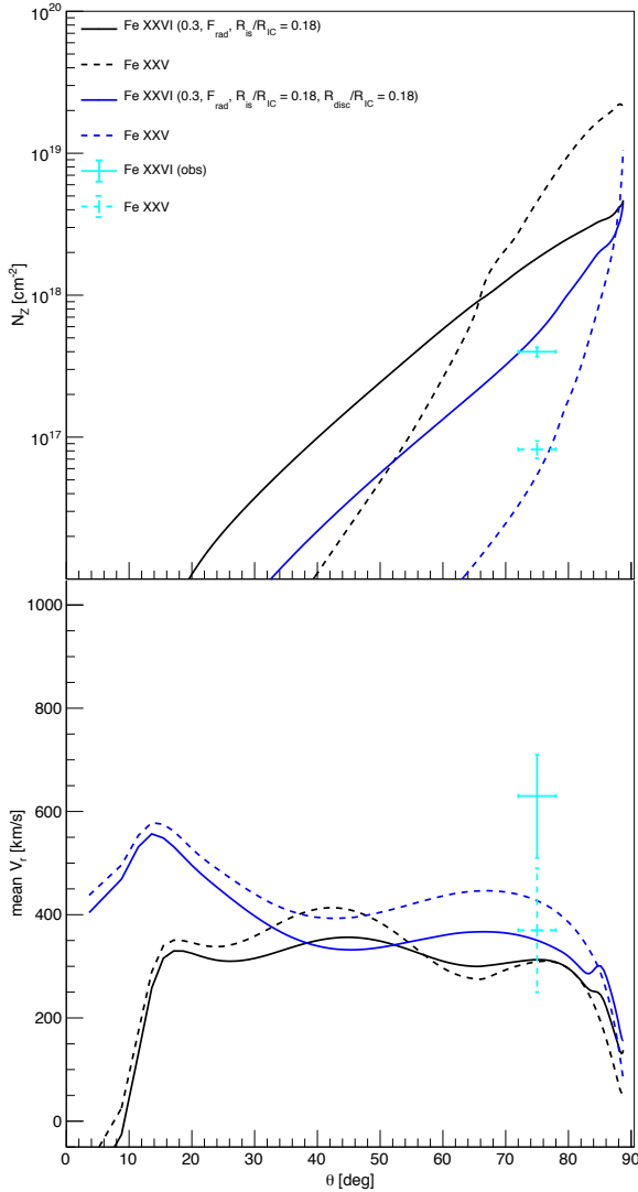
Figure 5. As in Fig. 4 but R_{\text{disc}}/R_{\text{IC}} = 1.0 (black) and 0.18 (blue).
