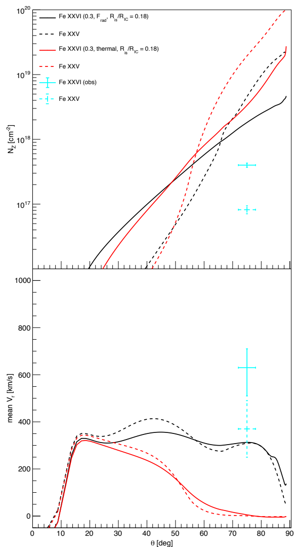
Figure 4. Top : the inclination dependence of column densities of Fe xxvi (solid line) and Fe xxv (dashed line). Bottom: the the inclination dependence of column weighted mean velocities of Fe xxvi (solid line) and Fe xxv (dashed line). The colours show the thermal-radiative wind of L/L_{\text{Edd}} = 0.3 , R_{\text{IS}}/R_{\text{IC}} = 0.18 (black), the thermal wind (red).
