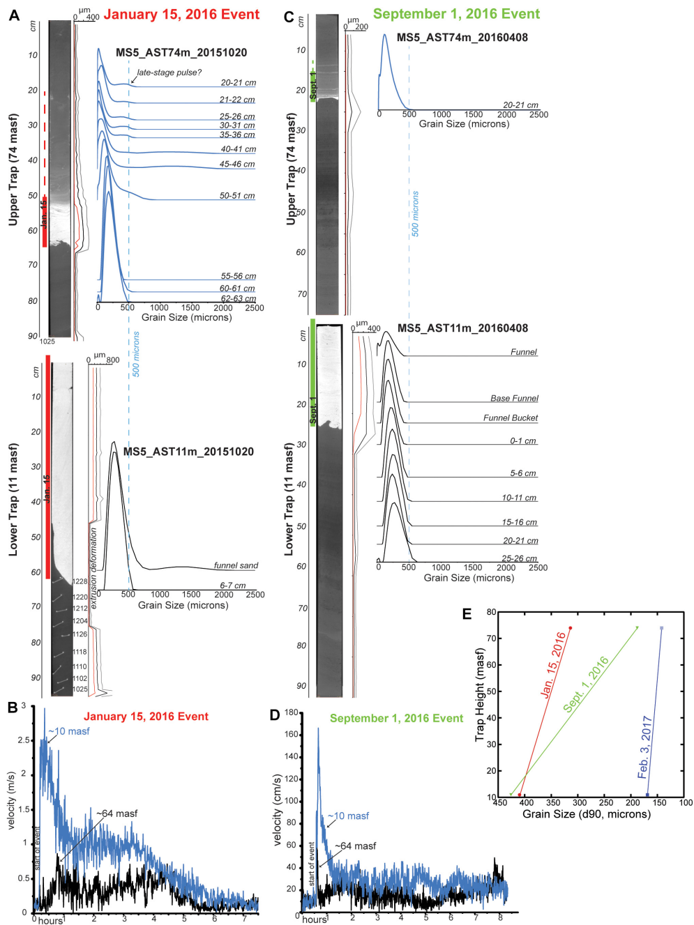
FIGURE 4 | Variation between traps at different heights above the seafloor. (A) January 15, 2016 sediment density flow event in mooring MS5 sediment traps at 11 m above the seafloor (masf) and 74 masf. Data shown as in Figure 3 (left), with additional grain-size distribution profiles within the January 15, 2016 event unit (right). (B) MS5 ADCP-measured velocity at 10 and 64 masf from the January 15, 2016 event. (C) September 1, 2016 sediment density flow event in MS5 sediment traps. Data shown as in (A) . (D) MS5 ADCP-measured velocity from the September 1, 2016 event, as in (B) . (E) d 0.9 grain size of coarsest extruded 1-cm samples from sediment density flow event units in MS5 sediment traps.
