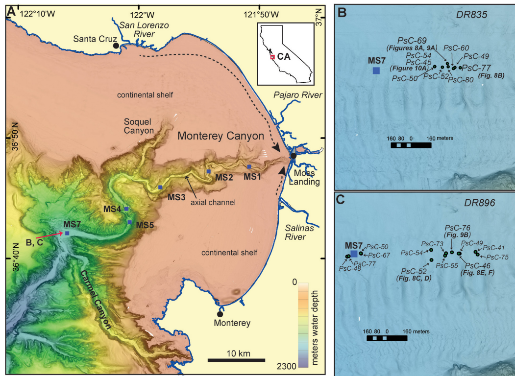
FIGURE 1 | Sample locations in Monterey Canyon, offshore central California. (A) Coordinated Canyon Experiment (CCE) moorings along Monterey Canyon axial channel (modified from Paull et al., 2018). Dashed arrows signify longshore transport of sand into Monterey Canyon. (B) Locations of remotely operate vehicle (ROV) pushcores from DR835, collected April 19, 2016 and plotted on Monterey Bay Aquarium Research Institute (MBARI) mapping autonomous underwater vehicle (AUV) 1-m lateral resolution slope-shaded multibeam bathymetry acquired on April 18, 2016. (C) Locations of ROV pushcores from DR896, collected October 19, 2016 and plotted on MBARI AUV 1-m lateral resolution slope-shaded multibeam bathymetry acquired on December 6, 2016.
