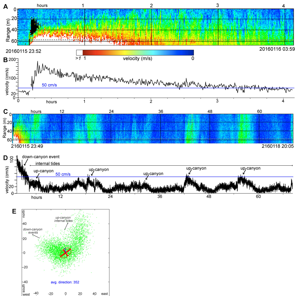
FIGURE 7 | Velocity during and following the January 15, 2016 event measured at MS7. (A) Color-contoured ADCP velocity panel. Range (y-axis) is shown as meters below the ADCP instrument, deployed at 65 m above the seafloor on mooring MS7. When the mooring is upright, the seafloor is at range 65 m, which is the base of this plot. (B) ADCP-measured velocity at approximately 10 m above the seafloor (masf) from (A) . (C) Color-contoured ADCP-measured velocity (labels as in A ), showing post-event internal tide variations. (D) Velocity profile from approximately 10 masf in (C) . (E) Scatter plot of MS7 velocity directions from 15 masf during Deployment I. Down-canyon internal tides and sediment density flow events are oriented primarily to the west-northwest, and up-canyon internal tides oriented primarily to the north-northeast.
