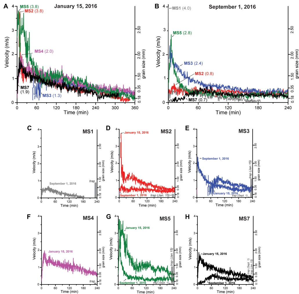
FIGURE 6 | Acoustic Doppler current profiler (ADCP)-measured velocity from approximately 10 m above the seafloor (masf; ADCP bin 055) adjacent to sediment trap samples at 10 masf. Grain size axes calculated after Komar (1985) and Ferguson and Church (2004). Velocity profiles in (A) from the January 15, 2016 event and (B) from the September 1, 2016 event, are labeled with mooring (MS#) and maximum ADCP-measured velocity (m/s) in each event at ~10 masf. Plots (C–H) show ADCP-measured velocities from each mooring and the range of measured d 0.1 to d 0.9 grain sizes in sediment traps from ~10 masf.
