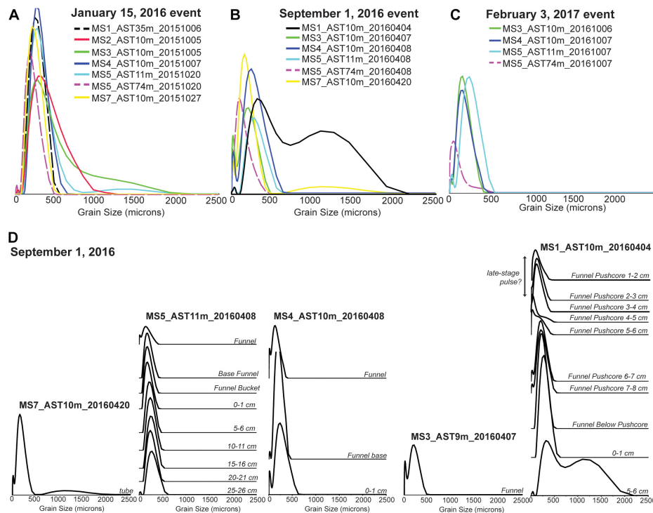
FIGURE 5 | Grain-size distributions from sediment density flow event units in sediment traps. Solid lines indicate samples from traps deployed at \sim 10 m above the seafloor (masf), and dashed lines indicate samples from traps deployed at > 10 masf. (A) January 15, 2016 event. (B) September 1, 2016 event. (C) February 3, 2017 event. (D) Stratigraphy of the September 1, 2016 event shown as grain-size distributions down-canyon (right to left, as in Figure 1).
