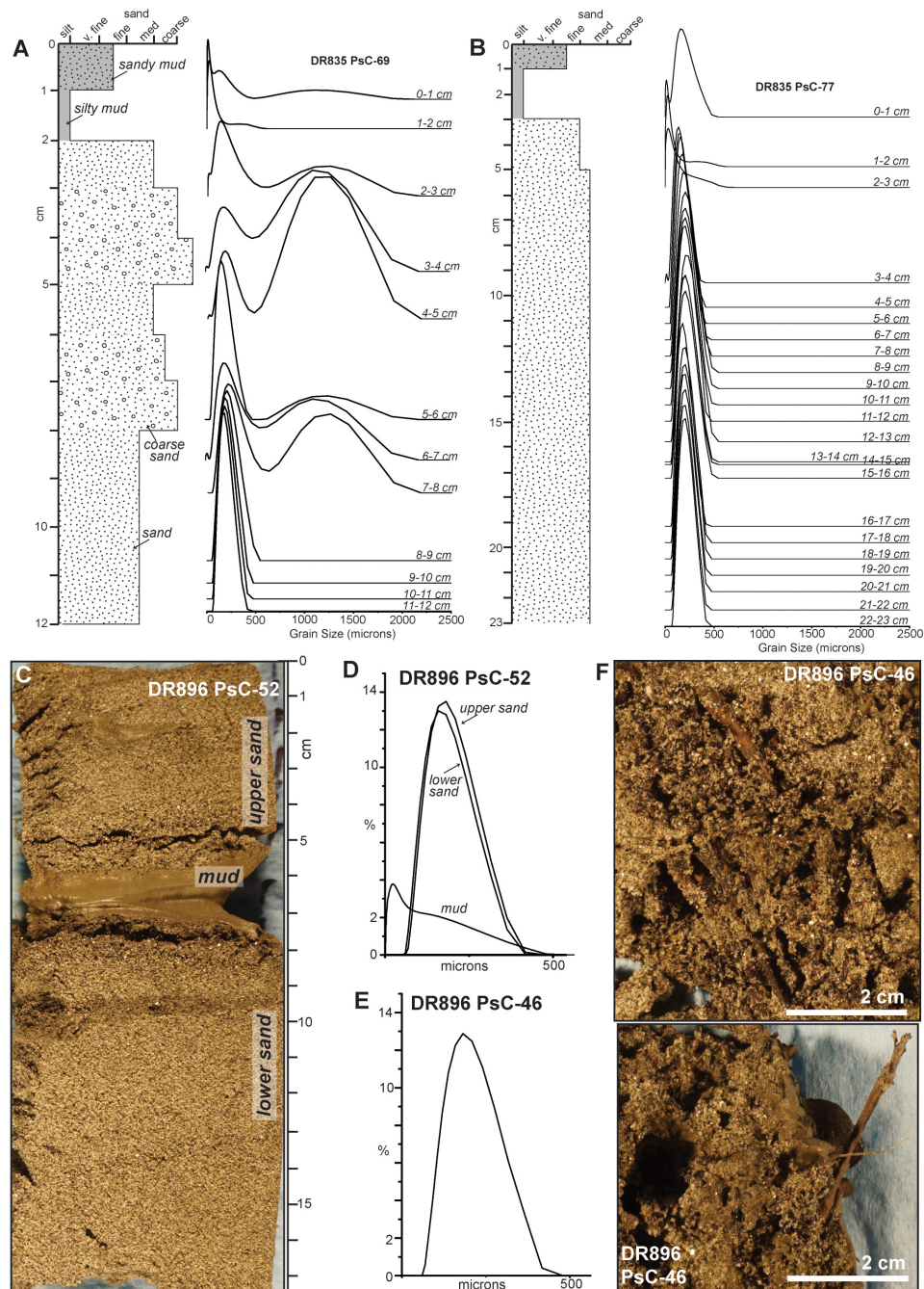
FIGURE 8 | Remotely operated vehicle (ROV) pushcore samples acquired near MS7. (A,B) Pushcores acquired in April 2016, following the January 15, 2016 event, shown as schematic log ( left ) and grain-size distributions ( right ). Stratigraphy and coarse grain size populations differ between these two closely spaced pushcores (57 m apart). See Figure 1B for sample locations. (C–F) Pushcores acquired in October 2016, after the September 1, 2016 event, shown as photographs and grain-size distributions. Woody plant material in sand is highlighted in (F) . See Figure 1C for sample locations.
