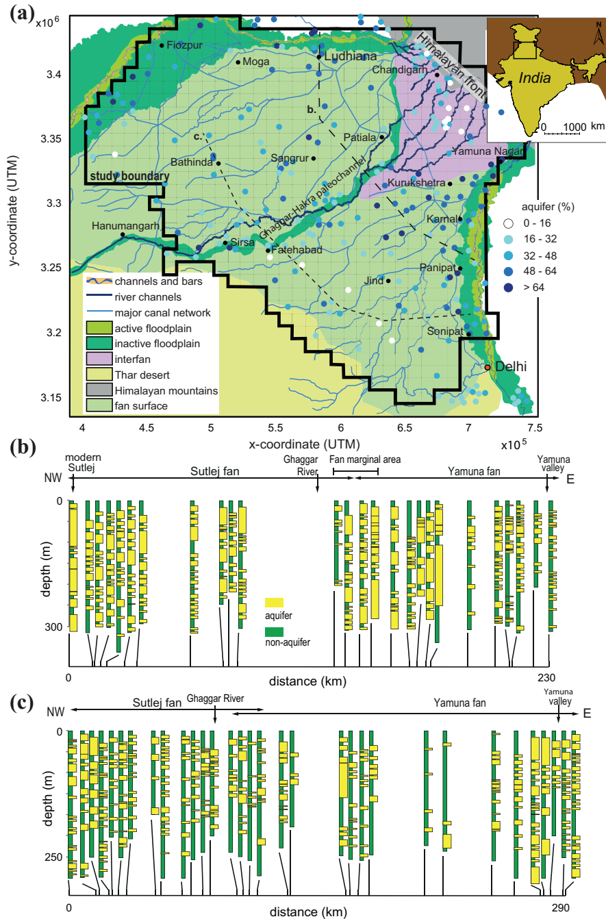
Figure 1. (a) Geomorphological map and the subsurface aquifer percentage of the study area in north-western India, modified after Van Dijk et al. (2016a). The study area covers the Sutelej and Yamuna fans (light green) and the interfan area between them (pink). Dark green areas show the incised valleys of the modern Sutelej and Yamuna rivers and the Ghaggar–Hakra paleochannel (Singh et al., 2017). Light blue lines show major canals. Dots show bulk aquifer percentage in the upper 200 m of the subsurface, based on CGWB
