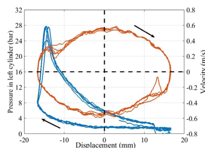
Figure 12. Cylinder pressure in the left cylinder with displacement (orange—velocity, blue—pressure in the left cylinder).
