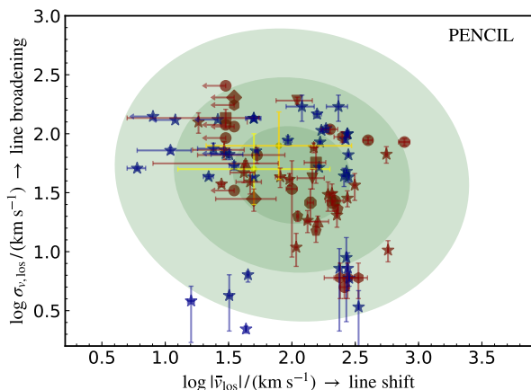
Figure 9. An analog to figure 4 of Gaspari et al. (2018) , showing the relation between the line of sight velocity dispersion (line broadening) and the magnitude of the line of sight velocity (line shift). This serves as a comparison between observational data and the predictions from chaotic cold accretion simulations ( 1-3\sigma green contours). The red and yellow points are observed systems with HI and CO clouds from Gaspari et al. (2018) , while the blue points show our ALMA detections from Table 5. The ALMA detections are statistically consistent with the distributions of previous data points and chaotic cold accretion predictions. It must be noted that we include detections of the same absorption regions from different molecular tracers because they likely trace different clouds or different parts of the giant molecular associations along the line of sight. Any emission seen is highly likely to originate from large collections of clouds, though absorption may well be detected due to single clouds along the line of sight.
