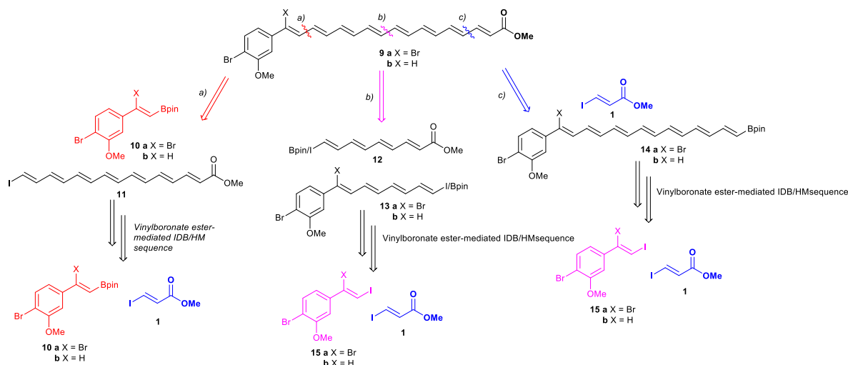
Scheme 2. Representative retrosyntheses of xanthomonadin and debromoxanthomonadin
