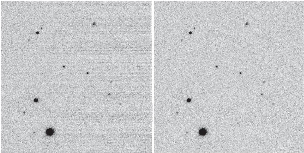
Figure 13. Correlated noise: example of the PATTERN.ROW correction on exposure o5379g0103o OTA57 cell xy01 ( i_{p1} filter 45 s). The left panel shows the cell with all appropriate detrending except the PATTERN.ROW, and the right shows the same cell with PATTERN.ROW applied. The correction reduces the correlated noise on the right side, which is most distant from the readout amplifier. There is a slight oversubtraction along the rows near the bright star.
