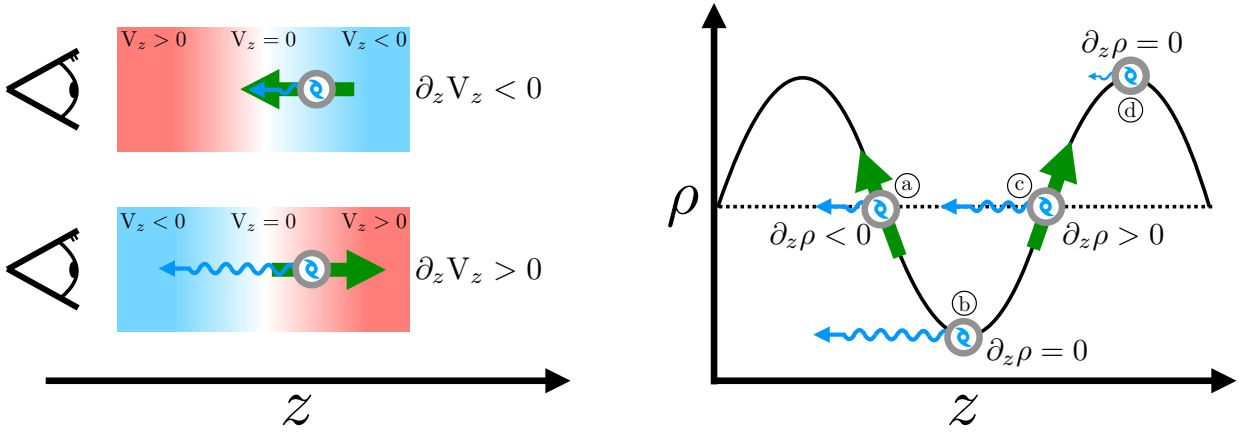
Figure 12. Schematic representation of the effect of density gradients. In this figure the observer is always at the left edge. Galaxies are represented as grey circles with a spiral inside. The green arrows indicate the gradient. Ly \alpha photons emitted toward the observer are shown with sinusoidal curves. The longer the photon arrows are, the higher the received flux and IGM transmission. Left: Illustration of the \partial_z V_z influence on the Ly \alpha observability. The background color maps represent IGM regions with a velocity gradient. The velocity along the line is color coded from negative (blue) to positive (red). Right: Cartoon of how the \rho and \partial_z \rho modify the Ly \alpha transmission. The dark line represents a density fluctuation along the line of sight.
