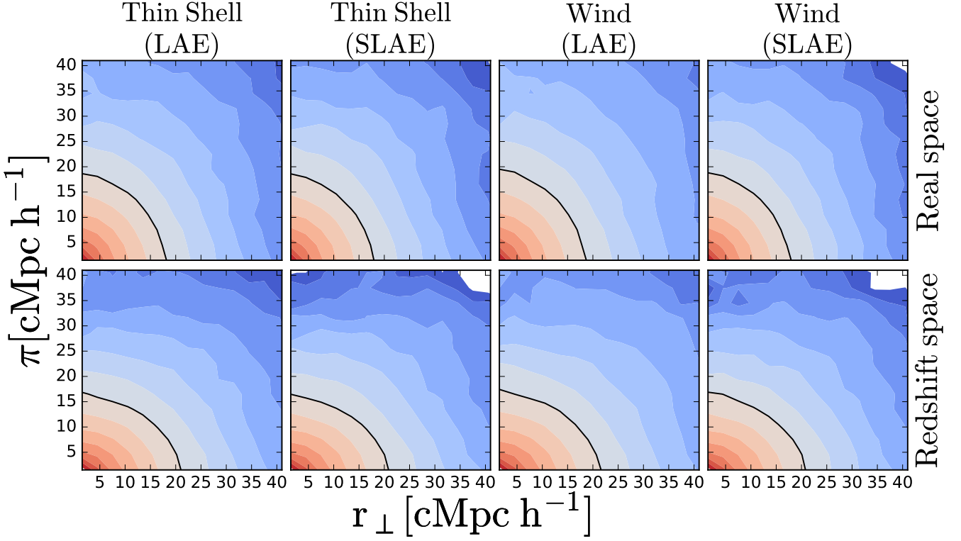
Figure 16. LAE 2-point correlation function as a function of parallel ( \pi ) and perpendicular ( r_{\perp} ) distance to the line of sight in real space (top) and redshift space (bottom) at redshifts 5.7. From left to right we show the FLAE Thin Shell, the SLAE Thin Shell, the FLAE Galactic Wind and the SLAE Galactic Wind. The contours are curves of iso-clustering amplitude, divided in 15 bins from \xi = 10^{0.5} to \xi = 10^{-2.5} equispaced in logarithmic scale and are color-coded coherently. Additionally, the black curve indicate \xi(\pi, r_{\perp}) = 0.01 .
