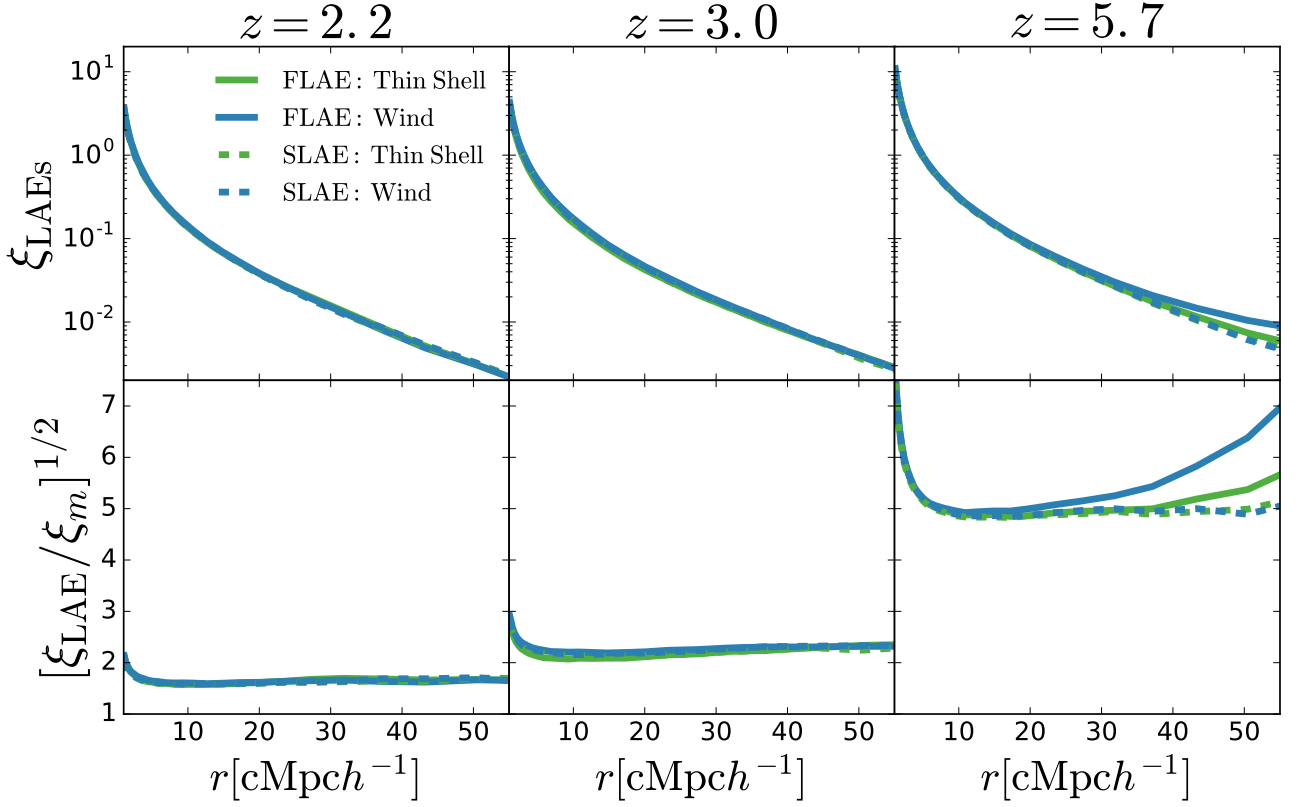
Figure 14. Top: 2-point Correlation function in real space for different samples at different redshifts (2.2, 3.0 and 5.7 from left to right). In dashed blue and green we show the SLAE Galactic Wind and Thin Shell respectively, while on the colors and solid line show the full RT models for the Galactic Wind and Thin Shell. Bottom: Bias of the different models as a function of distance.
