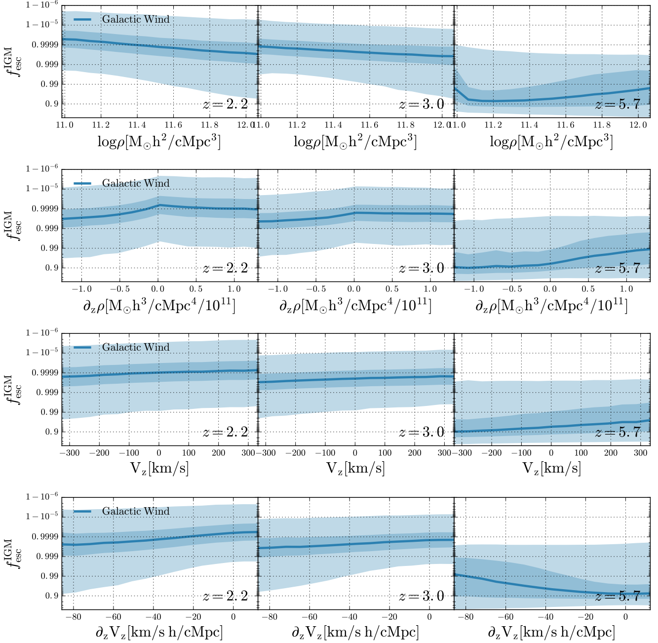
Figure 11. Same as Fig. 10 but for the Galactic Wind geometry.
