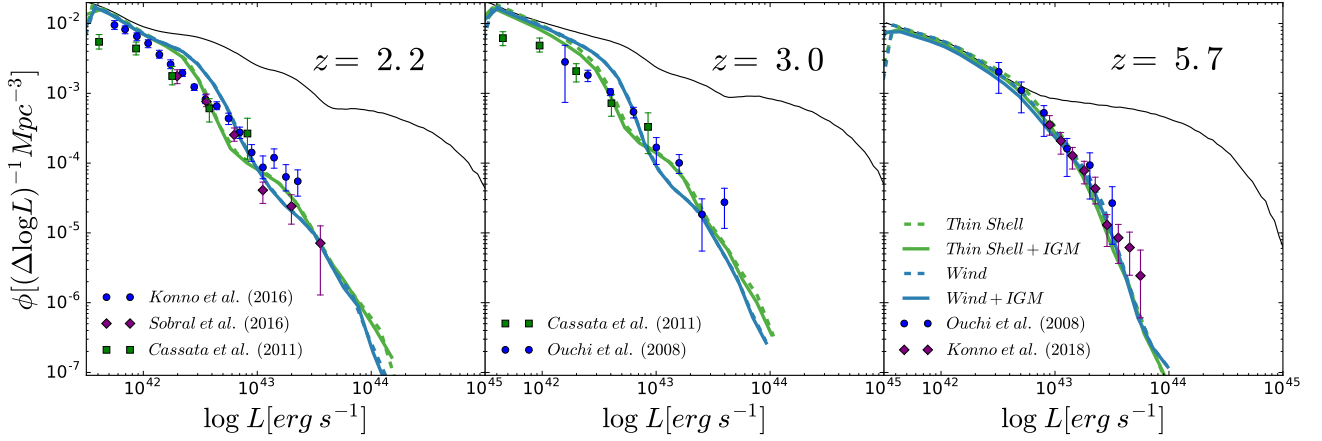
Figure 8. Comparison between our model's LAE luminosity function (LF) and observations at different redshifts. The intrinsic Ly \alpha LF is shown in thin black, the Thin Shell and Galactic Wind geometries are shown in green and blue dashed lines respectively. The colored dashed lines correspond to models with RT in the ISM but without RT in the IGM, while the colored solid lines include the RT in the ISM and IGM. Different observational data sets are shown in symbols according to the legends.
