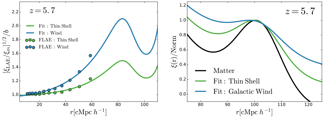
Figure 15. Left: Ratio between the bias as a function of distance and the median bias measured from 10 to 30 cMpch ^{-1} at redshift 5.7. In dots we show our simulation clustering while in solid curves the output of the MCMC analysis fitting the ZZ11 clustering description is illustrated. In blue and green we show the Galactic Wind and Thin Shell respectively. Right: Comparison of the 2PCF of our models and the matter 2PCF around the BAO peak. The clustering amplitudes are renormalized so that the maximum of the 2PCF between 90 and 110 cMpch ^{-1} match unity.
