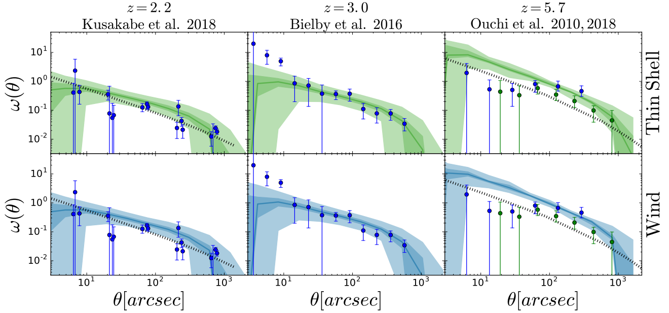
Figure 18. Comparison of the clustering of our models (full RT Thin Shell, full RT Galactic Wind from top to bottom) and different observational data set at redshift 2.2, 3.0 and 5.7 from left to right. At redshift 5.7, SILVERRUSH (Ouchi et al. 2018) is shown in blue dots while its predecessor (Ouchi et al. 2010) is plotted in green dots. The solid colored line indicated the median angular 2PCF of our mocks while the 1\sigma and 2\sigma are shown as shade regions. The different observations are shown as dots. Finally, the dashed black line indicate illustrate the best fitting clustering model presented within the original works.
