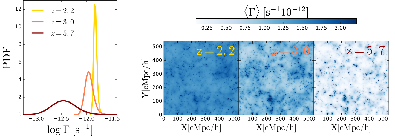
Figure 4. Left: Probability distribution function of the cosmic photoionization rate ( \Gamma ) at redshift 2.2 (yellow), 3.0 (orange) and 5.7 (brown). Right: Spatial distribution of the photoionization rate in different snapshots of the simulation (as labeled) in slices of \sim 2\text{cMpc}h^{-1} width.
