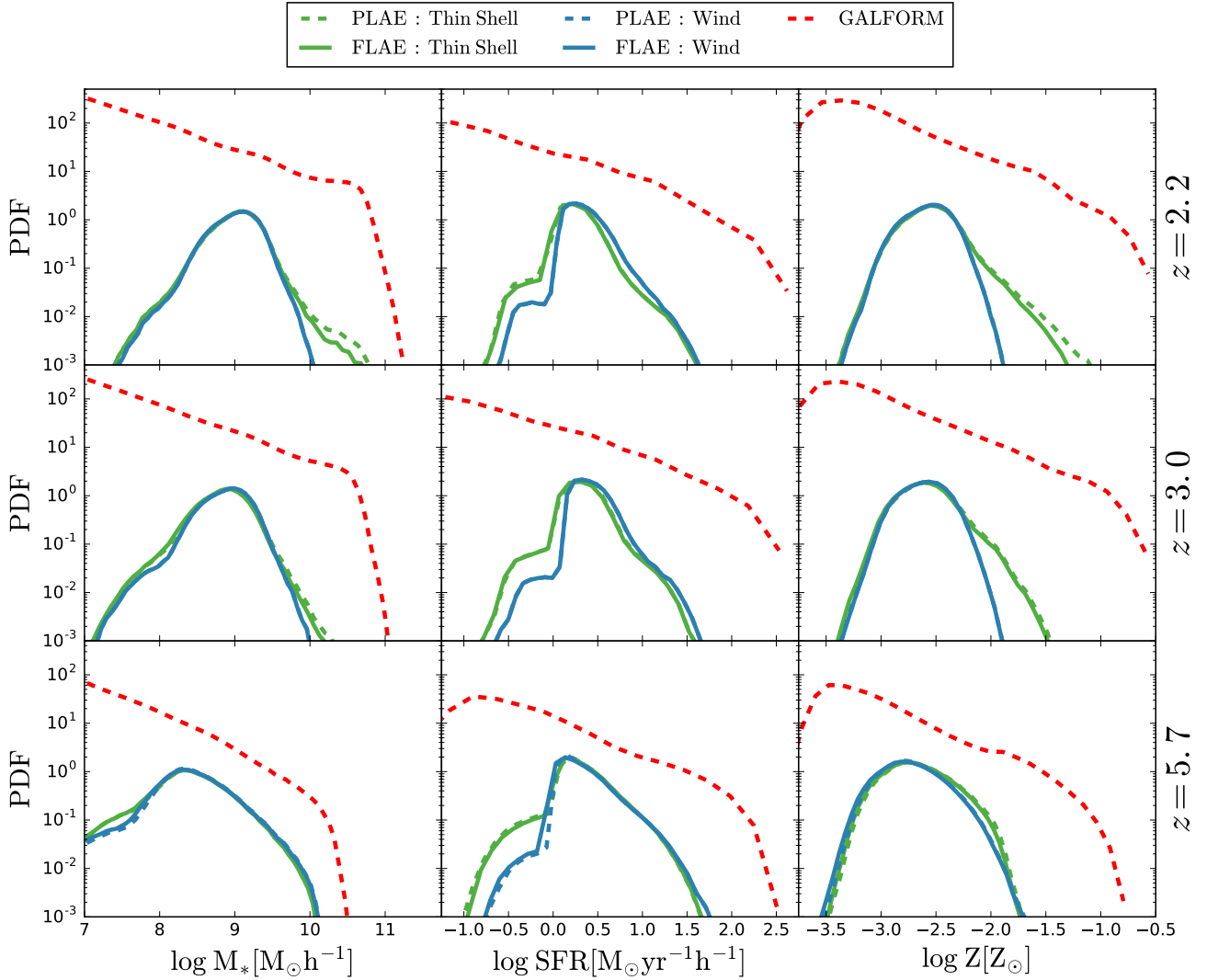
Figure 9. Comparison between the galaxy properties distribution (stellar mass, star formation rate and metallicity from left to right) of our different galaxy samples at several redshifts (2.2, 3.0, 5.7 from top to bottom). In dashed red we show the galaxy property distributions of the full GALFORM catalog. In dashed and solid green we display the galaxy properties distribution of the Thin Shell excluding and including the RT in the IGM. Meanwhile, blue shows the same as green but implementing the Galactic Wind geometry.
