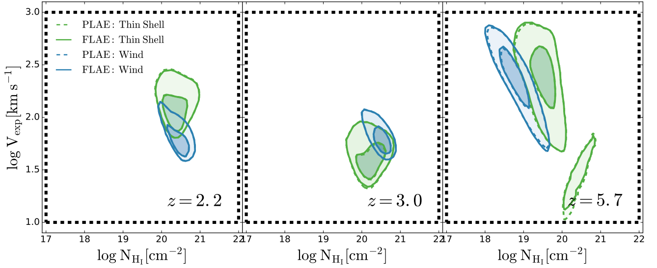
Figure A1. Distribution of LAE in the V_{\text{exp}}\text{-}N_{\text{HI}} space at redshift 2.2, 3.0 and 5.7 from left to right. The Thin Shell and Galactic Wind model are shown in green and blue. The dark contours represent the 1\sigma while the light the 2\sigma . The full RT models are shown in solid lines while the models with RT in the ISM but not in the IGM are plotted in dashed lines. In dashed black line we show FLAREON borders.
