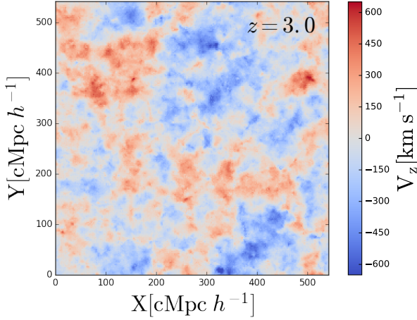
Figure 2. Velocity along the line of sight (Z axis) spatial distribution at redshift z = 3 in a slice of \sim 2\text{cMpc}h^{-1} width. Velocities pointing to the observer are shown in blue, while regions distancing from the observer are drawn in red.
