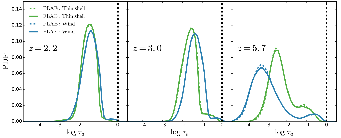
Figure A2. Distribution of the dust optical depth our models including RT in the ISM at redshift 2.2, 3.0 and 5.7 from left to right. The color code of the lines is the same as in Fig. A1.
