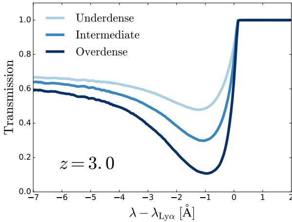
Figure 6. Median IGM transmission around the Ly \alpha wavelength for LAE samples hosted regions with different density. LAE living at the 1/3 of the lowest densities are shown in light blue, while in blue from the 1/3 to the 2/3 and dark blue for the LAE lying in the 1/3 densest environments.
