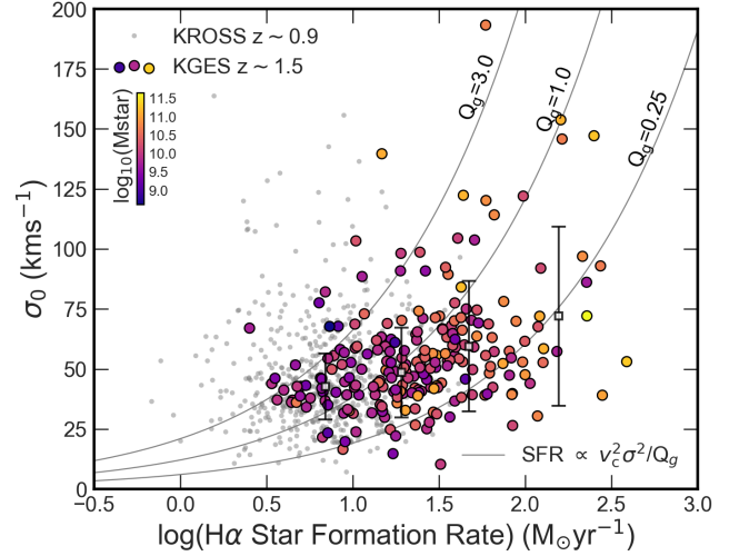
Figure 6. Velocity dispersion ( \sigma_0 ) as a function of the H\alpha star formation rate for KGES (coloured points) and KROSS (grey points) galaxies. KGES galaxies are coloured by their stellar mass ( M_* ) with the median and standard deviation of velocity dispersion in bins of H\alpha star formation rate shown by the square points. Galaxies of a higher star formation rate have higher stellar mass (Figure 2). We show the feedback driven turbulence model from Krumholz & Burkhardt (2016) for the relation between star formation rate and velocity dispersion, parameterised as \text{SFR} \propto v_c^2 \sigma^2 / Q_g , for different Toomre Q_g values, evaluated at the median rotational velocity of the KGES sample, \langle V_{2R_h} \rangle = 102 \pm 8 \text{ km s}^{-1} . The KGES galaxies occupy similar \sigma_0 – SFR parameter space as galaxies with Q_g = 0.25 - 3.0
