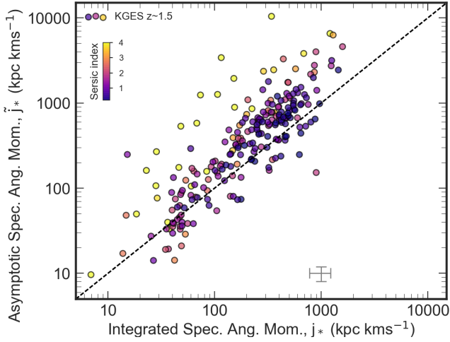
Figure 7. The asymptotic specific stellar angular momentum ( \tilde{j}_* ) as a function of the integrated specific angular momentum ( j_* ) evaluated at 2 \times half-stellar mass radius, for the KGES sample. The black dashed line indicates a one to one relation. The colour bar indicates the Sérsic index of the galaxy. The scatter below the line is a consequence of deconvolution with a broad-band PSF and convolution with the KMOS PSF. Scatter above the line is driven by galaxies of a higher Sérsic index in which the integrated specific angular momentum at 2 \times half-stellar mass radius is an underestimate of the total angular momentum in the galaxy.
