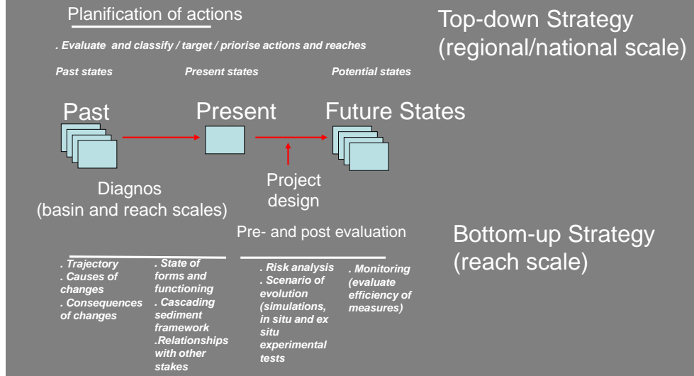
Figure 1. General framework of geomorphic studies: diagnosis and project appraisal, top-down and bottom-up strategies (From: Piégay et al. 2016, chapter 22)
