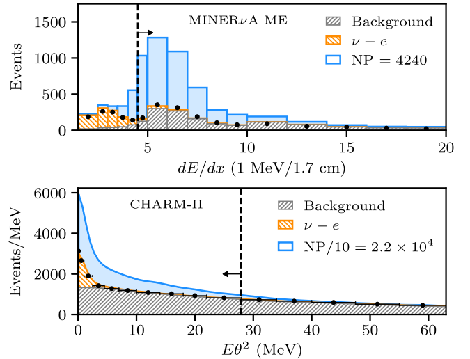
FIG. 2. New physics prediction at MINER \nu A ME and CHARM-II. Neutrino-electron scattering data in dE/dx at MINER \nu A (top) and in E\theta^2 at CHARM-II (bottom). Error bars are too small to be seen. For both experiments, we show the \nu - e signal and the total background prediction quoted (after tuning at MINER \nu A), as well as the NP prediction (divided by 10 at CHARM-II). The cuts in our analysis are shown as vertical lines.
