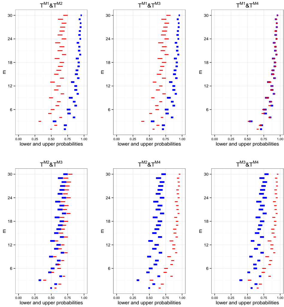
Figure 3: Pairwise comparisons of T^{M1} , T^{M2} , T^{M3} and T^{M4} , with \alpha = 0.5, \beta = 0.7 .
