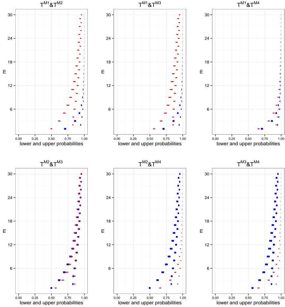
Figure 2: Pairwise comparisons of T^{M1} , T^{M2} , T^{M3} and T^{M4} , with \alpha = \beta = 0.5 .
