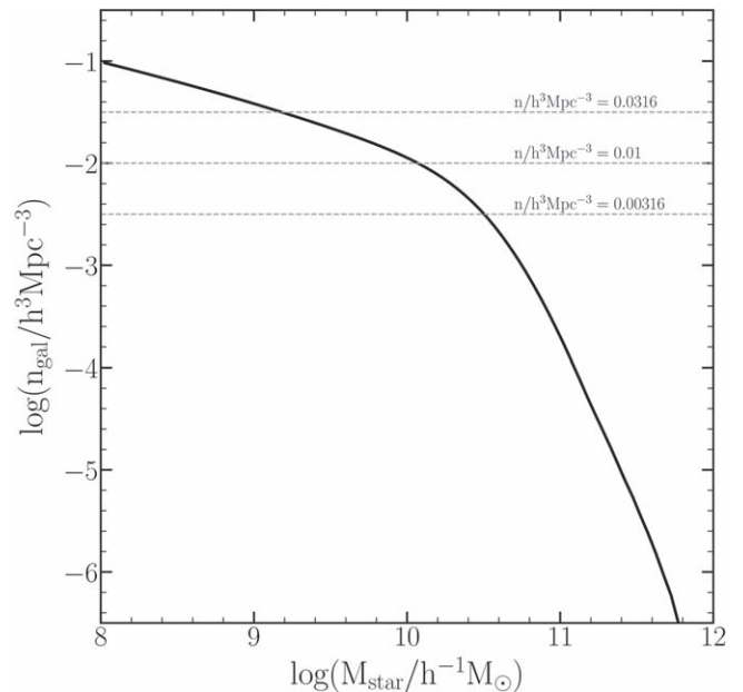
Figure 1. Cumulative stellar mass function predicted by the Guo et al. (2013) SAM. The dashed horizontal lines indicate the number densities of the samples used in this work.
