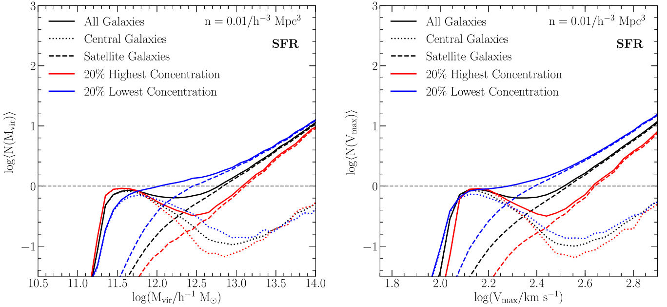
Figure 11. Occupancy variation with concentration for an SFR-selected sample corresponding to a number density of n = 0.01 h^3 \text{Mpc}^{-3} , shown for M_{\text{vir}} (left) and V_{\text{max}} (right).
