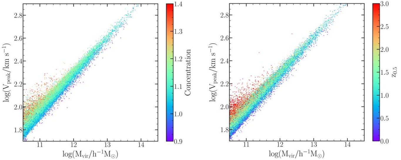
Figure 14. Relation between V_{\text{peak}} and M_{\text{vir}} color coded by halo concentration (left) and by halo formation time (right). These are the analog of Figure 2 but for V_{\text{peak}} instead of V_{\text{max}} . For clarity, we plot a representative (randomly chosen and ordered) 1% of the halos.
