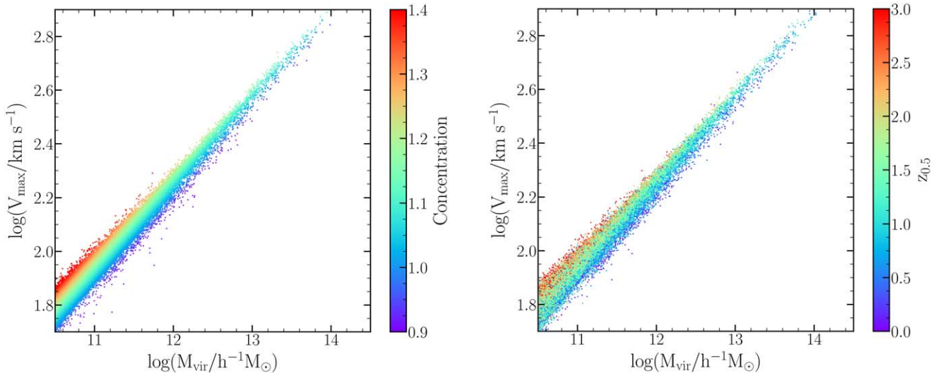
Figure 2. Relation between V_{\max} and M_{\text{vir}} , color coded by halo concentration (left) and by halo formation time (right). For clarity and to avoid overcrowding, we plot only 1% of the halos randomly chosen and ordered.
