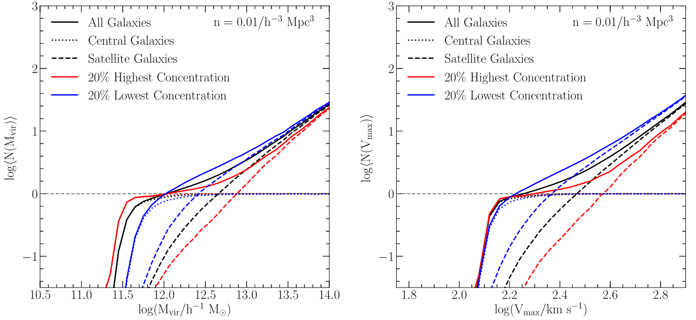
Figure 3. Halo occupation functions for the n = 0.01 h^3 \text{ Mpc}^{-3} galaxy sample, for the full galaxy sample (black), for the galaxies in the 20% most concentrated halos (red), and 20% least concentrated halos (blue). The occupation functions are shown as a function of M_{\text{vir}} on the left and V_{\text{max}} on the right.
