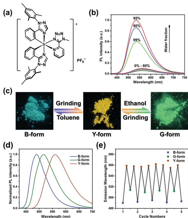
Fig. 1 (a) Chemical structure of complex 1 . (b) Normalized emission spectra of complex 1 in CH 3 CN–H 2 O mixtures (complex concentration = 5.0 \times 10^{-5} M) with different water fractions (0–99% v/v) at room temperature. (c) Photographs and schematic representation of a tricolour luminescence switching process. (d) Normalized emission spectra of B-, G- and Y-forms. (e) Repeated cycles of the tricolour luminescence switching process.
