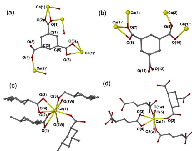
Figure 3. (a) The binding of ligand CHTCA to the calcium ions in [\text{Ca}_3(\text{C}_9\text{H}_9\text{O}_6)_2(\text{H}_2\text{O})_4] \cdot 3\text{H}_2\text{O} ( 5 ), and (b) [\text{Ca}(\text{C}_9\text{H}_{10}\text{O}_6)(\text{H}_2\text{O})_2] \cdot \text{H}_2\text{O} ( 6 ). Selected interatomic distances in 5 (Å): \text{Ca}(1)-\text{Ca}(2) = 3.836 , \text{Ca}(1)-\text{Ca}(1') = 9.492 , \text{Ca}(1')-\text{Ca}(2') = 8.044 . Selected bond lengths in 6 (Å): \text{Ca}(1)-\text{Ca}(2) = 5.095 , \text{Ca}(1')-\text{Ca}(1'') = 9.377 , \text{Ca}(1)-\text{Ca}(1') = 4.001 , \text{Ca}(1'')-\text{Ca}(2) = 5.192 . (c) The calcium coordination environment in [\text{Ca}(\text{C}_9\text{H}_{10}\text{O}_6)(\text{H}_2\text{O})_2] \cdot \text{H}_2\text{O} ( 6 ); (d) the calcium coordination environment in [\text{Ca}(\text{C}_9\text{H}_{10}\text{O}_6)(\text{H}_2\text{O})_2] \cdot 0.5\text{H}_2\text{O} ( 7 ).
