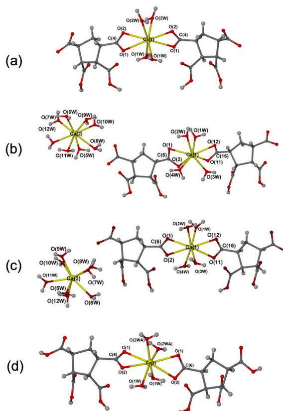
Figure 2. Calcium complexes of CPTCA. (a) Structure of [\text{Ca}(\mu\text{-C}_9\text{H}_8\text{O}_8)(\text{H}_2\text{O})_4]_n ( 1 ) 16 ; (b) structure of [\text{Ca}(\text{H}_2\text{O})_8][\text{Ca}(\text{C}_9\text{H}_8\text{O}_8)_2(\text{H}_2\text{O})_4] \cdot 2\text{H}_2\text{O} ( 2 ); (c) structure of [\text{Ca}(\text{H}_2\text{O})_8][\text{Ca}(\text{C}_9\text{H}_8\text{O}_8)_2(\text{H}_2\text{O})_4] ( 3 ); (d) structure of [\text{Ca}(\text{C}_9\text{H}_8\text{O}_8)_2(\text{H}_2\text{O})_4]_n ( 4 ).
