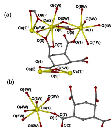
Figure 4. Crystal structures of [\text{Ca}_2(\text{C}_{10}\text{H}_8\text{O}_8)(\text{H}_2\text{O})_7] \cdot 2\text{H}_2\text{O} ( 8 ) and [\text{Ca}(\text{C}_{10}\text{H}_{10}\text{O}_8)(\text{H}_2\text{O})_6] \cdot \text{H}_2\text{O} ( 9 )
