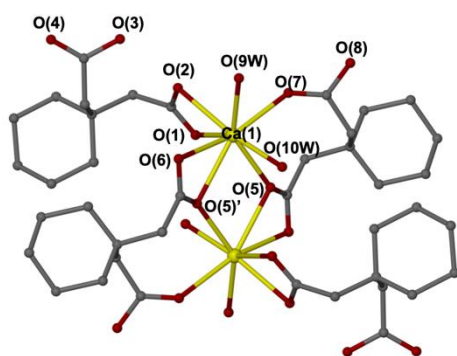
Figure 5. The crystal structure of [\text{Ca}(\text{C}_{10}\text{H}_{15}\text{O}_4)_2(\text{H}_2\text{O})_2]_n ( 13 ), shows the eightfold coordination.
