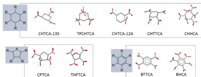
Figure 6. The orientation of the COOH along the cyclic 6-membered ring, 5-membered ring and benzene ring. TPCHTCA(DEVCOV); 24 THFTCA (ZEZLEV); 25 BTTCa (PYMELL12); 26 BHCA (MELLIT). 27
