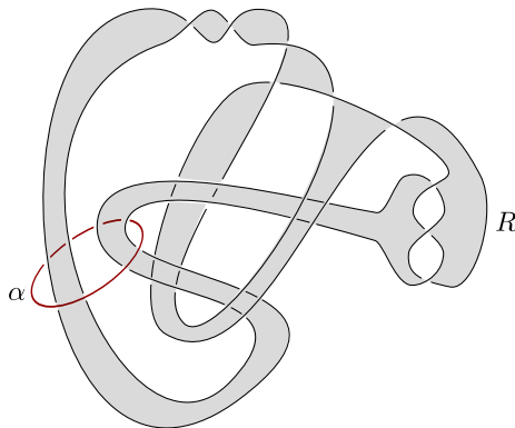
FIGURE 1. The knot R = 8_8 with a grey Seifert surface and a red infection curve \alpha .
