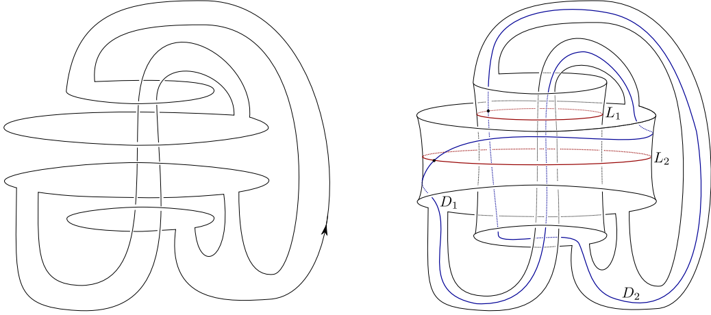
FIGURE 2. The knot R = 11_{n74} = P(3, -3, 3, -2) (left) and a Seifert surface for R along with two derivative links L = L_1 \cup L_2 and D = D_1 \cup D_2 (right).
