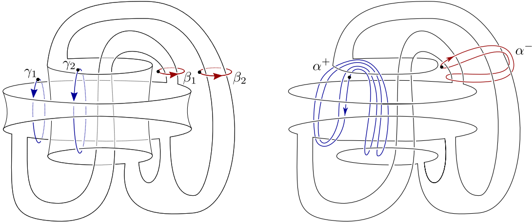
FIGURE 3. Unknotted curves \beta_1, \beta_2, \gamma_1, \gamma_2 in \pi_1(M_R)^{(1)} (left) and \alpha^\pm in \pi_1(M_R)^{(2)} (right).
