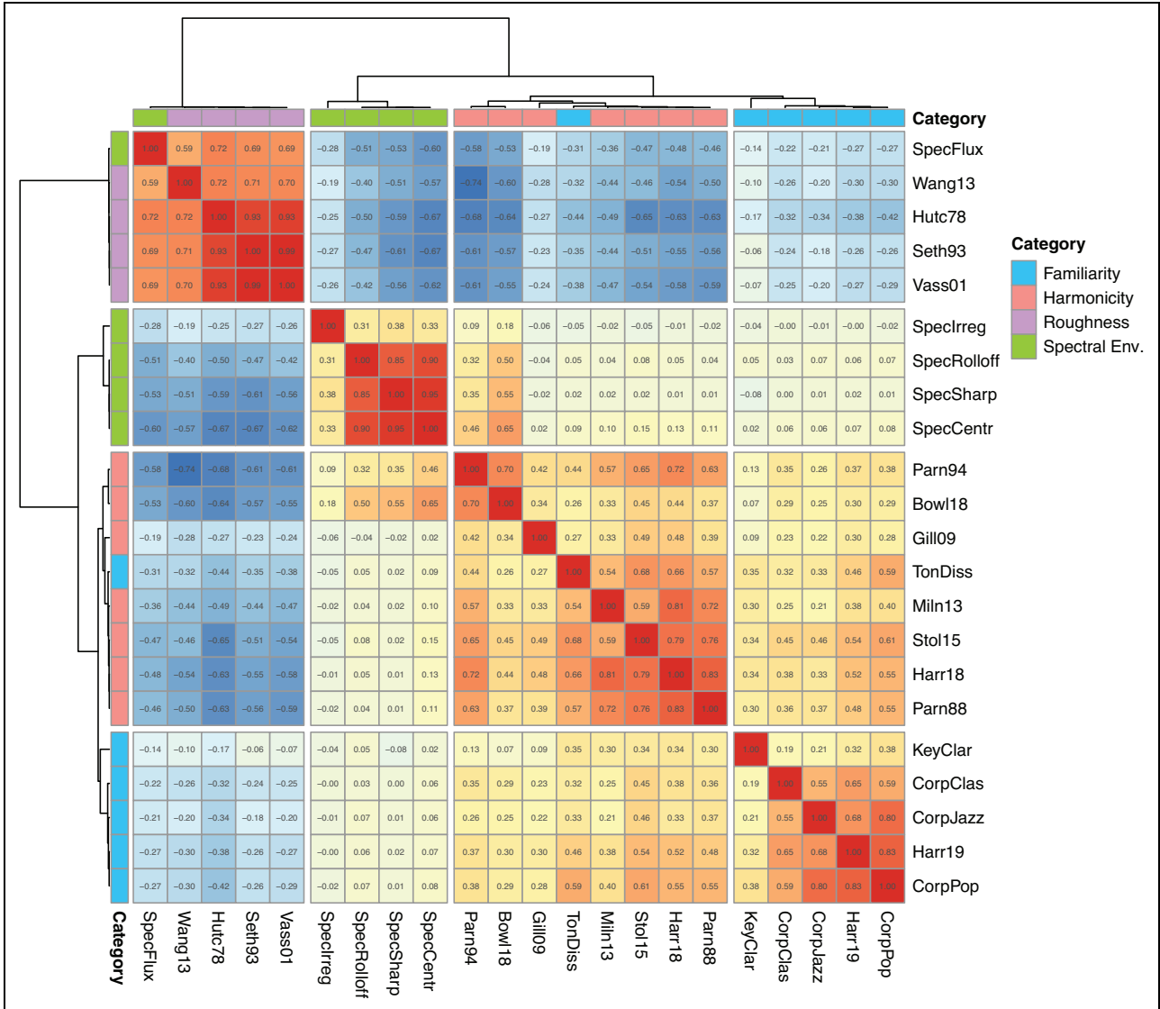
Figure 1. Correlations and a hierarchical cluster solution for predictors of roughness, harmonicity, familiarity, and spectral envelope categories (Durham Chord Dataset, n = 4755 ).
