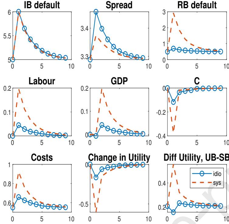
Fig 2. IB (investment bank) default, Spread, RB (retail bank) default, Costs/GDP are in % values. Labour, GDP, C (Consumption) are log deviation from steady-state. "Change in utility" is difference in consumption equivalent from steady-state. Difference in utility UB-SB is between universal and separated banking in consumption equivalent for a given shock.
