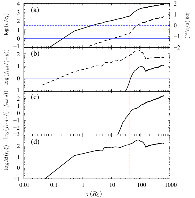
Figure 4. The velocity (panel a), the radiation force normalized by the gravity (panel b), the ratio of the radiation force to the \theta -component of the radiation force to the r -component (panel c), and the force multiplier (panel d) on the major wind streamline (blue line in Fig. 1). The horizontal axis is the distance from the z = 0 plane. In the panel a, the velocity is normalized by the sound speed (solid line) and by the escape velocity (dashed line). The solid line in the panel b shows the r -component of the radiation force, and the \theta -component is presented by the dashed line. The wind matter mainly moves vertically at z \lesssim 40R_S (left side of red dashed-dotted line), and is blown away in the radial direction at z \gtrsim 40R_S (right side of red dashed-dotted line).
