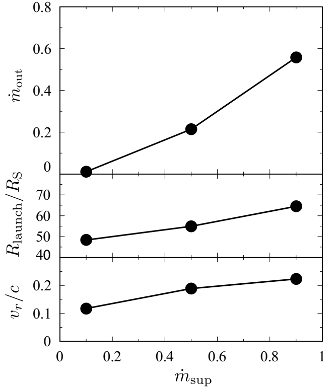
Figure 6. Wind mass loss rate (panel a), launching radius (panel b), and averaged radial velocity weighted by the density (bottom panel c) as functions the mass supply rate. The black hole mass and the X-ray fraction are M_{\text{BH}} = 10^8 M_\odot and f_X = 0.2, 0.04, 0.02 for \dot{m} = 0.1, 0.5, 0.9 .
