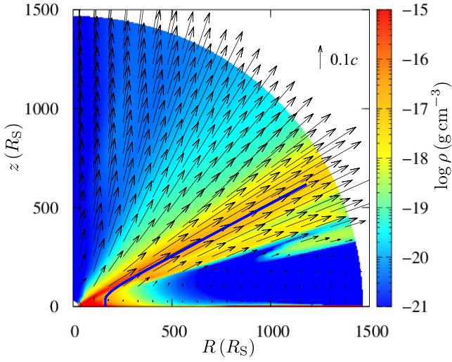
Figure 1. Time-averaged colour density map with the velocity vectors of the line-driven disc wind for M_{\text{BH}} = 10^8 M_{\odot} , \dot{m}_{\text{sup}} = 0.5 , and f_{\text{X}} = 0.1 . The blue line shows a streamline through the mainstream (streamline passing through \rho v_r peak at the outer boundary) of the wind. The z = 0 plane roughly corresponds to the accretion disc surface and the z -axis is the rotational axis of the disc.
