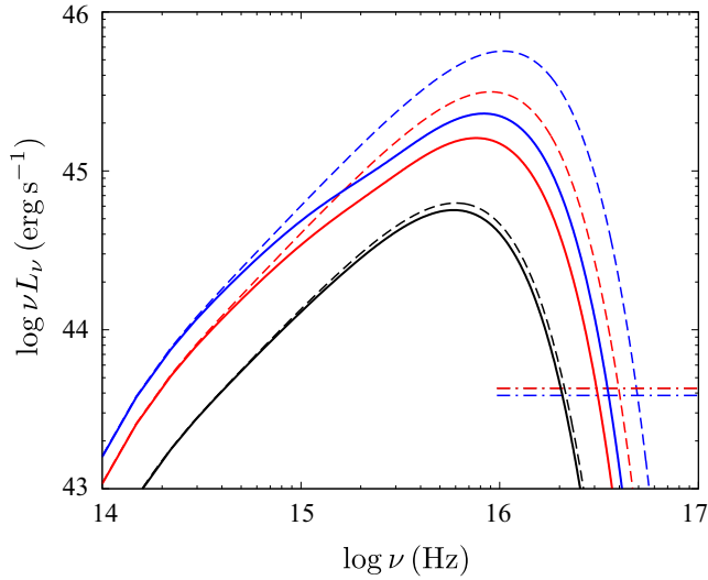
Figure 7. SEDs of the radiation from the accretion discs when we set M_{\text{BH}} = 10^8 M_{\odot} . The black, red, and blue solid lines show the SEDs for \dot{m}_{\text{sup}} = 0.1, 0.5, and 0.9 of our mass-conserved simulations. The black, red, and blue dashed lines are the SEDs of the standard disc model with \dot{m}_{\text{sup}} = 0.1, 0.5, and 0.9 . The black, red, and blue dot-dashed lines are the X-ray spectra employing the power-law spectrum with a photon index of \Gamma = 2 . The X-ray fractions are f_{\text{X}} = 0.2, 0.04, and 0.02 for \dot{m}_{\text{sup}} = 0.1, 0.5, and 0.9 .
