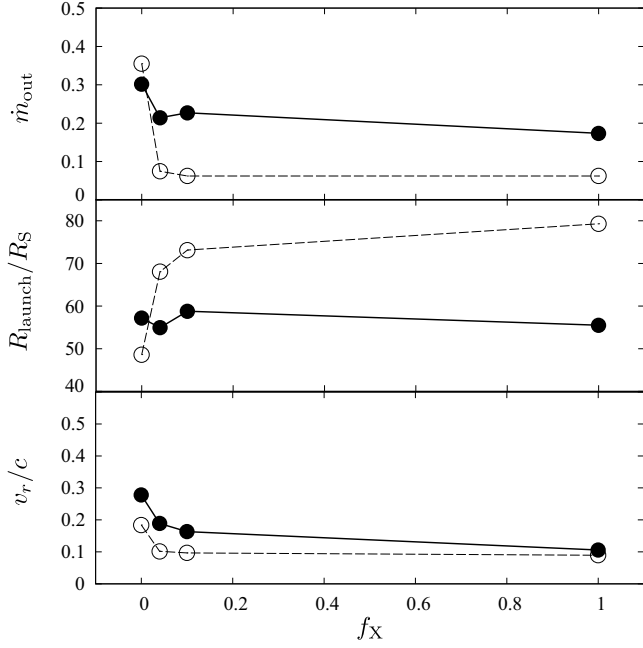
Figure 5. Wind mass loss rate (top panel), launching radius (middle panel), and averaged radial velocity weighted by the density (bottom panel) as functions of X-ray fraction, f_X . We employ M_{\text{BH}} = 10^8 M_\odot and \dot{m}_{\text{sup}} = 0.5 for f_X = 0, 0.04, 0.1 and 1 . The filled circles show the results when we employ \sigma_X = \sigma_e for \xi > 10^5 and 100\sigma_X for \xi \leq 10^5 . The open circles indicate the results using \sigma_X = \sigma_e independently of \xi and ignoring the attenuation of the UV line-driving flux.
