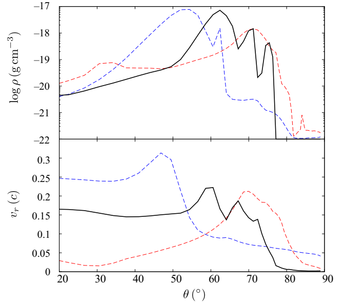
Figure 2. Angular profiles of the density (top panel) and the radial velocity (bottom panel) at the outer boundary ( r = 1500R_{\text{S}} ). The black solid lines show the profiles for the new mass-conserved simulations with \dot{m}_{\text{sup}} = 0.5 ( \dot{m}_{\text{BH}} \sim 0.26 ). The red dashed, and blue dashed lines show the profiles for the constant accretion rate models with \dot{m}_{\text{sup}} = 0.2 , and \dot{m}_{\text{sup}} = 0.5 .
