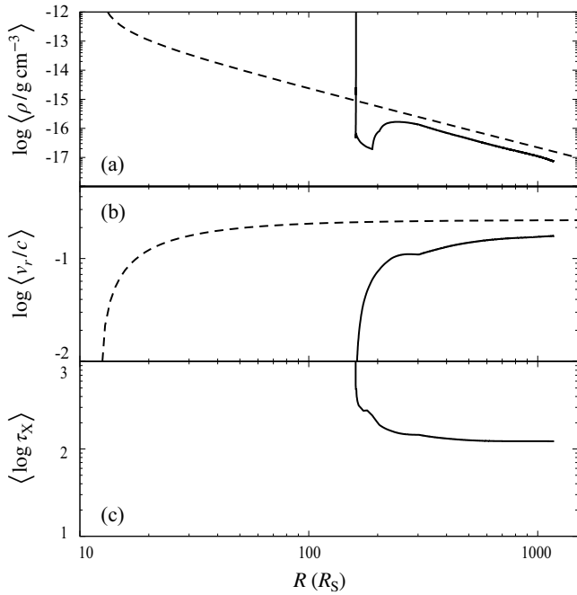
Figure 3. Density (panel a), velocity (panel b), and optical depth to the central X-ray source (panel c) along the streamline. The angle brackets denote the time-averaged values. The horizontal axis is the distance from the rotational axis of the disc. The solid lines show the results along the mainstream (blue line in Fig. 1) of our simulations for M_{\text{BH}} = 10^8 M_{\odot} , \dot{m}_{\text{sup}} = 0.5 , and f_X = 0.1 . The dashed lines show the expectations from the phenomenological model of Hagino et al. (2015) with the wind terminal velocity of v_{\infty} = 0.237c and the mass loss rate of 8 M_{\odot} \text{yr}^{-1} .
