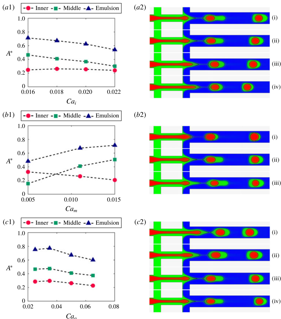
FIGURE 11. Inner part, middle part and the entire double emulsion size variations in the periodic one-step formation regime (regime 8) by changing: (a1) Ca_i = 0.016, 0.018, 0.02 and 0.022 at Ca_m = 0.011 and Ca_o = 0.05 ; (b1) Ca_m = 0.005, 0.011 and 0.015 at Ca_i = 0.018 and Ca_o = 0.05 ; (c1) Ca_o = 0.025, 0.035, 0.05 and 0.065 at Ca_i = 0.018 and Ca_m = 0.011 . The snapshots shown in (a2-i-a2-iv), (b2-i-b2-iii) and (c2-i-c2-iv) correspond to the flow conditions mentioned in (a1-c1).
