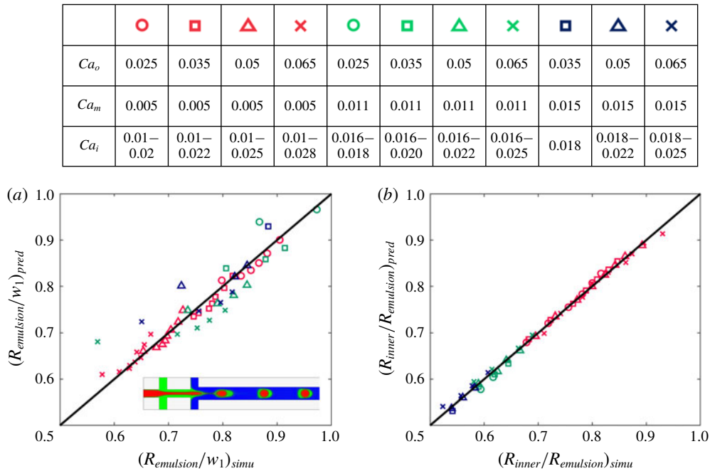
FIGURE 12. The parity plots of (a) the normalized entire double emulsion radius (R_{emulsion}/w_1)_{pred} computed from (4.2) and the simulated values of (R_{emulsion}/w_1)_{simu} ; (b) the radius ratio of the inner part to the entire double emulsion (R_{inner}/R_{emulsion})_{pred} computed from (4.3) and the simulated values of (R_{inner}/R_{emulsion})_{simu} . The points in both plots are based on all periodic one-step flow conditions (regime 8) obtained in figure 6. The legend table shows that the flow conditions of all feasible Ca_i at each Ca_m and Ca_o combination are represented by symbols of the same type, and the values of Ca_m and Ca_o are differentiated through the symbol colours and shapes, respectively. The inset in subfigure (a) shows the snapshot of one typical periodic one-step formation regime at Ca_i = 0.02 , Ca_m = 0.011 and Ca_o = 0.05 .
