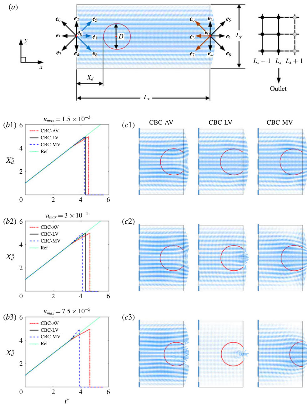
FIGURE 2. (a) Illustration of the moving droplet set-up; (b1–b3) time histories of X_d^* for u_{max} = 1.5 \times 10^{-3} , 3.0 \times 10^{-4} and 7.5 \times 10^{-5} with different convective boundary conditions; (c1–c3) typical snapshots of the droplet shape and velocity vectors when the droplet passes through the outlet layer with each CBC boundary at u_{max} corresponding to (b1–b3), respectively. The X_d and time values are normalized using X_d^* = X_d/D and t^* = tu_{max}/D .
