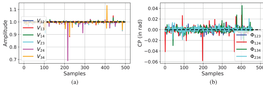
Fig. 10. Retrieved simulated visibilities with four input beams coupled into the DBC device. Both the amplitudes and phases vary following a statistical Gaussian distribution (see text for details). Black is the theoretical curve. (a) Visibility amplitudes. (b) Closure phases.
