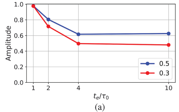
Fig. 13. Median value of the retrieved visibility amplitude ( V_{14} ) as a function of the exposure time. The legend shows the Strehl ratio. Here the case n = 1 assumes t_e = 30\text{ ms} with N_p = 10^4 photons per pixel.
