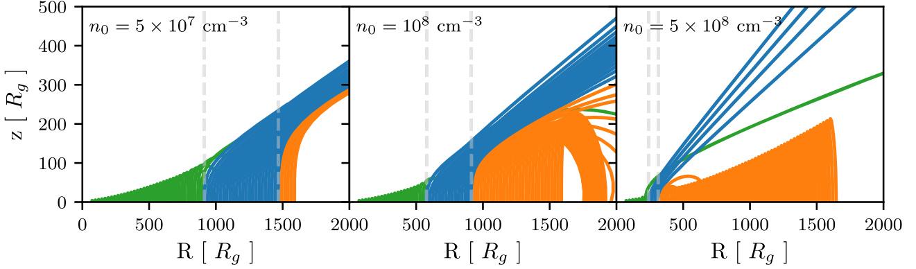
Figure 9. Three wind simulations from the parameter range scan shown in Fig. 8. The initial velocity is fixed to v_0 = 10^8 cm/s, while the initial density is varied in the range n_0 \in (5 \times 10^7, 10^8, 5 \times 10^8) cm ^{-3} . Higher density values shift the escaping region to smaller radii, thus reducing the effective disc surface that produces an escaping wind. Furthermore, the increase in UV shielding narrows the range of escaping streamlines. Note that a high number of streamlines was used to produce Fig. 8, according to the rule in equation (22), but we plot only a fraction of them for clarity.
