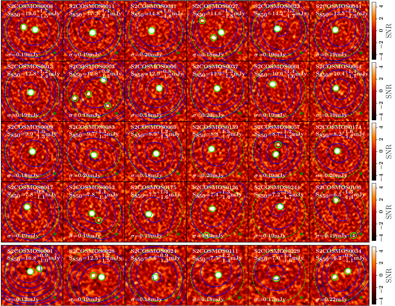
Figure 1. Thirty example ALMA 870- \mu\text{m} continuum maps, displayed as signal-to-noise ratio maps from \pm 5 \sigma , from our pilot survey of the 182 brightest SCUBA-2-identified sources in the COSMOS field. The top four rows were selected at random from our 160 Cycle 4 ALMA targets in bins of single-dish flux density (in descending flux from the top row: S_{850\mu\text{m}} = 13\text{--}20 , 10\text{--}13 , 8\text{--}10 , 6\text{--}8 mJy). Our AS2COSMOS pilot survey includes 24 archival ALMA maps and we show a randomly-chosen subset of these in the final row to highlight that they have a comparable quality to our Cycle 4 data. We detect 260 SMGs (circled) at > 4.8 \sigma across the 182 ALMA 870 \mu\text{m} maps, with flux densities of 0.7–19.2 mJy. The presence of multiple continuum counterparts in a fraction of the maps is clear (e.g., S2COSMOS 0003, see §3.3). Solid contours represent SCUBA-2 emission at 4, 6, 8, 12, 16, 20, and 24 \sigma . The panels are 20 \times 20'' ( 160 \times 160 kpc at z \sim 2.5 ), the dashed circle represents the 17.3'' primary beam of ALMA at 870 \mu\text{m} and we show the synthesized beam in the bottom right of each map, as well as a colour bar indicating the signal-to-noise scaling on the right of each row.
