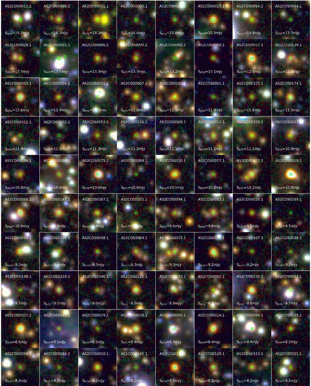
Figure 4. 20'' \times 20'' images showing the K_s , 3.6 \mu\text{m} & 4.5 \mu\text{m} (corresponding to BGR channels) colour images for the 80 brightest 870- \mu\text{m} SMGs ( S_{870\mu\text{m}} \geq 8.1 mJy) in the AS2COSMOS sample (the remaining SMGs are shown in Fig. A1). Each image is centred on the ALMA source position and are ordered by decreasing ALMA 870- \mu\text{m} flux density. Contours represent the ALMA 870 \mu\text{m} detections are overlaid at 4, 10, 20, and 50 \sigma . These images demonstrate that the AS2COSMOS SMGs are typically very red and/or faint at near-to-mid infrared wavelengths, relative to the field population. We find that 9 \pm 1 per cent of the AS2COSMOS SMGs are not detected in the Ultravista/ K_s imaging, at the > 5 \sigma significance level, but note that all but one of these sources are detected in the deblended IRAC imaging (median m_{4.5} = 23.5 \pm 0.2 ). Overall, the AS2COSMOS SMGs have a median K_s - 4.5 \mu\text{m} colour of 1.24 \pm 0.04 mag, reflecting the importance of sensitive mid-infrared imaging for conducting an unbiased study in to the stellar emission of 870 \mu\text{m} -luminous sources.
