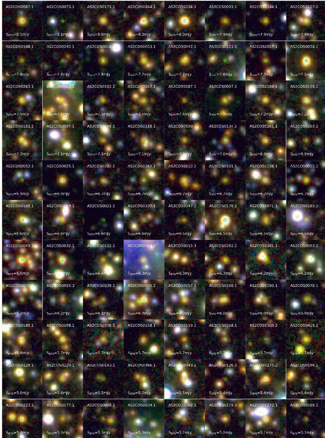
Figure A1. 20'' \times 20'' images showing the K_s , 3.6 \mu\text{m} & 4.5 \mu\text{m} (corresponding to BGR channels) colour images of the faintest 180/260 ASCOSMOS SMGs, those with S_{870\mu\text{m}} \leq 8.5 \text{ mJy} . Each image is centred on the ALMA source position and are ordered by decreasing ALMA 870\text{-}\mu\text{m} flux density. Contours represent the ALMA 870 \mu\text{m} detections are overlaid at 4, 10, 20, and 50 \sigma . Along with the brighter SMGs shown in Figure 4, these images demonstrate that the ASCOSMOS SMGs are typically very red and/or faint at near-to-mid infrared wavelengths, relative to the field population. We note that the apparent frequency of ALMA-detected companions in the fields of the fainter sources is simply a result of these sources being so faint that they are only included in our sample if they lie in close proximity to a brighter SMG.
