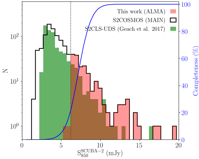
Figure 2. The 850\ \mu\text{m} flux density distribution of the 182 single-dish-identified sources that comprise our ALMA-S2COSMOS pilot study, compared to the parent distribution of S2COSMOS MAIN sources. The AS2COSMOS pilot survey is effectively complete for S2COSMOS sources brighter than 6.2\ \text{mJy} (182/183; dotted line). For comparison, we show the flux distribution for the S2CLS-UDS sample of SCUBA-2-identified sources (Geach et al. 2017), the parent sample for a similar ALMA follow-up study (AS2UDS; Stach et al. 2019), to demonstrate that AS2COSMOS has roughly twice the source numbers at S_{850\ \mu\text{m}} > 6.2\ \text{mJy} , relative to a comparable, degree-scale survey. The solid curve represents the effective completeness of the AS2COSMOS pilot survey after accounting for incompleteness in AS2COSMOS and S2COSMOS studies, as well as the effect of a fixed selection at S_{850\ \mu\text{m}} > 6.2\ \text{mJy} on the S2COSMOS catalogue. AS2COSMOS is estimated to be 22, 50 and 90 per cent complete to sources at S_{850\ \mu\text{m}} = 6.2, 7.2 and 8.9\ \text{mJy} , respectively, across a survey area of 1.6\ \text{deg}^2 .
