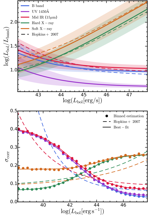
Figure 2. Top: Bolometric corrections as a function of bolometric quasar luminosity. We show the bolometric corrections in the rest-frame B band, UV, mid-IR, soft and hard X-ray determined by our fiducial quasar mean SED template. 1\sigma dispersions are shown with shaded region. The bolometric corrections in Hopkins et al. (2007) are shown in dashed lines. Bottom: Magnitude of the dispersions in bolometric corrections as a function of bolometric quasar luminosity. Both binned estimations and best-fit relations are presented.
