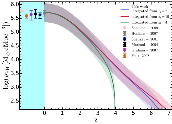
Figure 12. Predicted evolution of the cosmic SMBH mass density at z = 0-7 . The red, blue and green lines represent the predictions with starting redshift of integration z_i = 10, 7, 4 respectively. We assume the averaged radiative efficiency \epsilon_r = 0.1 . Shaded regions show the uncertainties when increasing or decreasing \epsilon_r by 2 times. The data points show the estimated SMBH mass density in the local Universe from Shankar et al. (2004) ; Marconi et al. (2004) ; Graham & Driver (2007) ; Yu & Lu (2008) ; Shankar et al. (2009) . The local SMBH mass density is mainly dominated by the SMBH growth at z < 4 .
