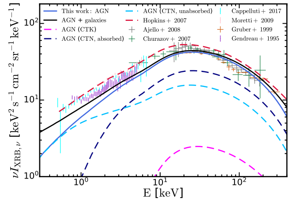
Figure 11. Predicted CXB spectrum. The prediction from our global best-fit model, which only includes the contribution from quasars, is shown with the blue solid line. The prediction that accounts for a simplified constant 2 \text{ keV}^2 \text{ s}^{-1} \text{ sr}^{-1} \text{ keV}^{-1} contribution from galaxies is shown with the black solid line. The predictions that only include CTK ( \log N_{\text{H}} \geq 24 ) or absorbed CTN ( 22 \leq \log N_{\text{H}} \leq 24 ) or unabsorbed CTN AGN ( \log N_{\text{H}} \leq 22 ) are shown in dashed lines. We compare the predictions to the measurements from Gendreau et al. (1995); Gruber et al. (1999); Churazov et al. (2007); Ajello et al. (2008); Moretti et al. (2009); Cappelluti et al. (2017). We also show the prediction from the Hopkins et al. (2007) model with the red dashed line. The prediction from this work is generally in agreement with the observations despite a \sim 0.05 dex lower at E \lesssim 20 \text{ keV} .
