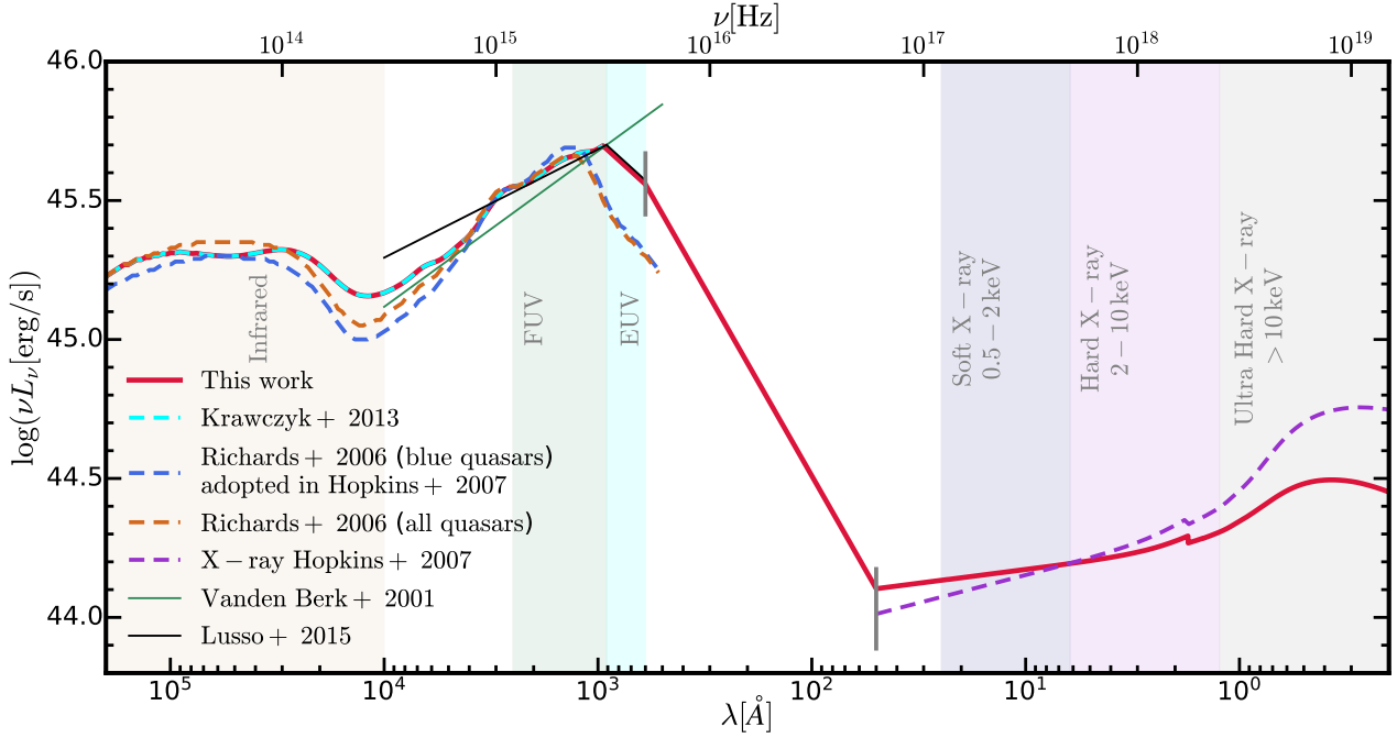
Figure 1. Mean SED template of quasars constructed in this work. The template SED shown here has the normalization \nu L_\nu \approx 45.5 \text{ erg s}^{-1} at 2500\text{\AA} . The solid red line represents our fiducial SED model. SED templates from other works are presented: Richards et al. (2006b), the blue and orange dashed lines; Hopkins et al. (2007) X-ray SED, the purple dashed line; Krawczyk et al. (2013), the cyan dashed line. The power-law models for optical/UV SED are shown in the green (Vanden Berk et al. 2001) and black (Lusso et al. 2015) thin lines. The common bands for the measurements of quasar luminosities are shown with shaded regions. In this paper, the bolometric luminosity is defined as the integrated luminosity from 30\mu\text{m} to 500\text{keV} .
