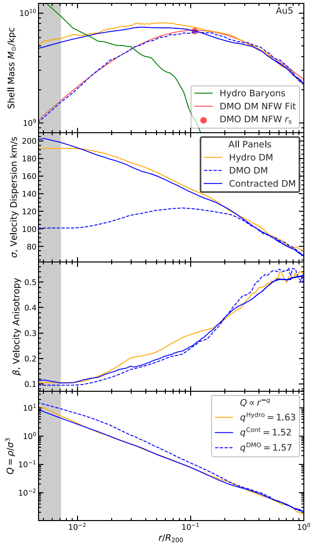
Figure 2. An illustration of the density, velocity dispersion, and velocity anisotropy profiles of a DM halo (AURIGA halo 5) shown for the DMO (dashed blue) and the Hydro (solid orange) versions of the simulation. Compared to the DMO case, the Hydro halo has a higher density in the central regions (top panel), along with an increased velocity dispersion (second panel). The third panel shows only small differences in the velocity anisotropy, \beta . The bottom panel shows the pseudo-phase-space density, Q(r) = \rho/\sigma^3 , which we find is well fitted by a simple power law for both DMO and Hydro haloes. Also plotted is the contracted DMO halo (solid blue), which was obtained by applying the method described in Section 3.1. This closely reproduces the Hydro halo. The grey shaded region corresponds to r values below the convergence radius of the simulation (Power et al. 2003).
