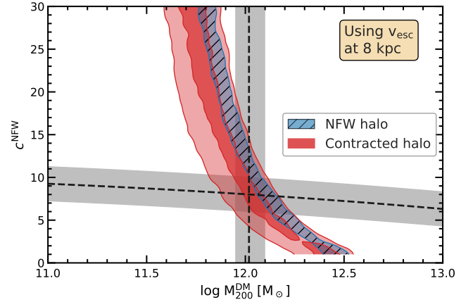
Figure 9. Constraints on the mass and concentration of the MW DM halo inferred from the escape velocity measurement of Deason, Fattahi, Belokurov, Evans, Grand, Marinacci & Pakmor (2019) . The blue shaded region shows the 68 percentile confidence region when modelling the halo as an NFW profile. The red shaded regions show the 68 and 95 percentile contours when taking into account the contraction of the Galactic DM halo – in this case the concentration corresponds to the value before applying the baryonic contraction. The dashed lines and grey shaded regions are as in Figure 8.
