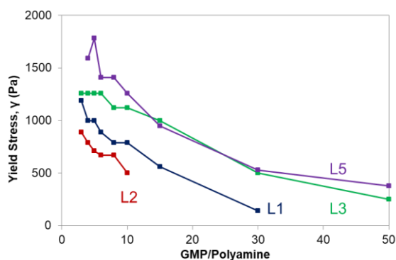
Figure 5. Plot of the yield stress as a function of the GMP/polyamine quotient.
