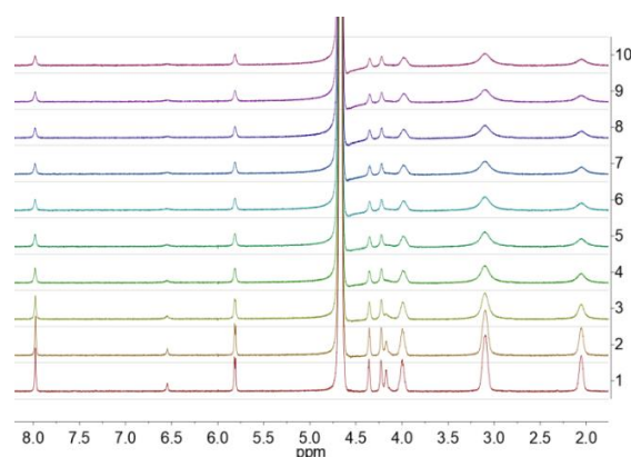
Figure 7. ^1\text{H} NMR spectra recorded during the GMP-L5 hydrogel formation kinetic studies. Spectra were recorded every 25 seconds. The study was performed employing the optimal conditions for the GMP-L5 hydrogel formation: GMP:L5 5:1 molar ratio.
