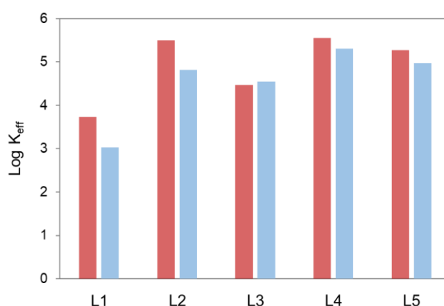
Figure 2. Plot of the values of the logarithms of the effective constants for the interaction of L1-L5 with GMP at pH 5.0 (red) and pH 7.4 (blue). [L1-L5] = [GMP] = 1.0 \cdot 10^{-3} M.
