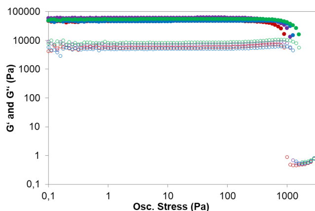
Figure 4. Oscillatory stress sweep experiments for the optimal conditions for the gelation for each GMP-polyamine system. G' : Filled circles. G'' : Empty circles. GMP:L1 3:1 (purple). GMP:L2 3:1 (red). GMP:L3 4:1 (blue). GMP:L5 5:1 (green).
