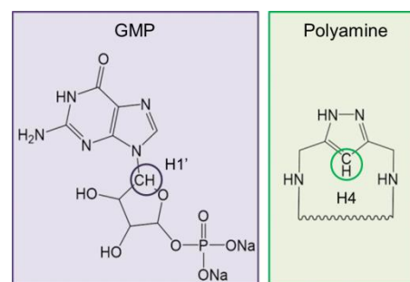
Figure 6. ^1\text{H} NMR monitored signals during the kinetic studies of the GMP-polyamine gel formation.
