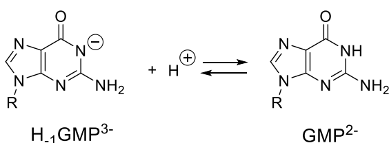
Scheme 1. Protonation equilibrium of the GMP imidic nitrogen. Taking into account the basicity of ligands and GMP, the cumulative stability constants obtained with the aid of
