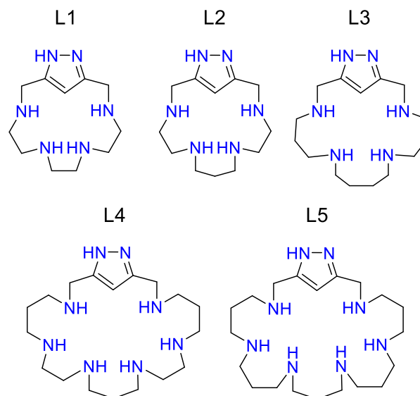
Figure 1. 1 H -pyrazole azamacrocycles L1-L5 .
