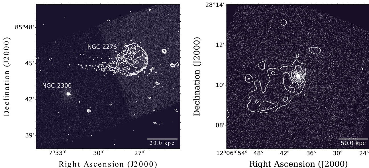
Figure 7. Left-hand panel: Overlay of LOFAR contours on the Chandra X-ray image, showing together NGC 2300 and NGC 2276. For the LOFAR image, the first contour is at 0.00075\text{mJy beam}^{-1} , and each contour increases by a factor of two. Right-hand panel: Overlay of LOFAR contours of the diffuse emission on the Chandra X-ray image in NGC 4104, where the first contour is at 0.0002\text{mJy beam}^{-1} , and each contour increases by a factor of two.
