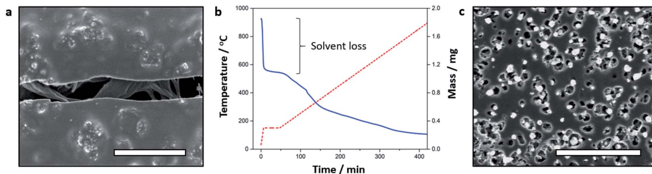
Fig. 7 (a) SEM micrograph of fibres in desiccation cracks of a typical dried lily pad aggregate coated in 2 nm platinum (scale bar 1\text{ }\mu\text{m} ); (b) TGA thermogram for a lily pad aggregate undergoing pyrolysis in nitrogen; (c) SEM micrograph of an uncoated lily pad aggregate pyrolysate (scale bar 1\text{ }\mu\text{m} ).
