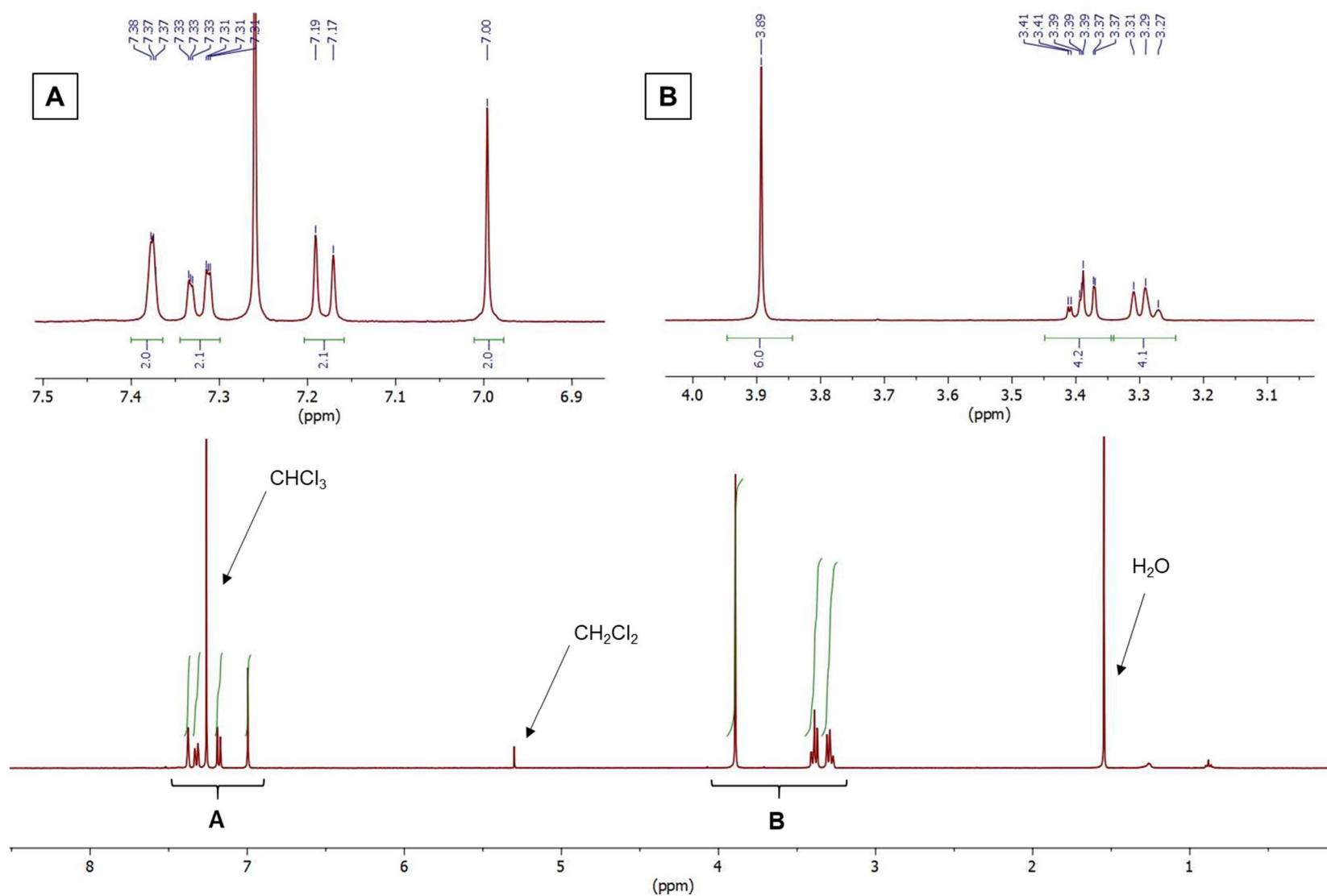
Figure 2. 1 H NMR spectrum of OPE3-Ph(OMe) 2 (400 MHz, CDCl 3 at 25 °C).
