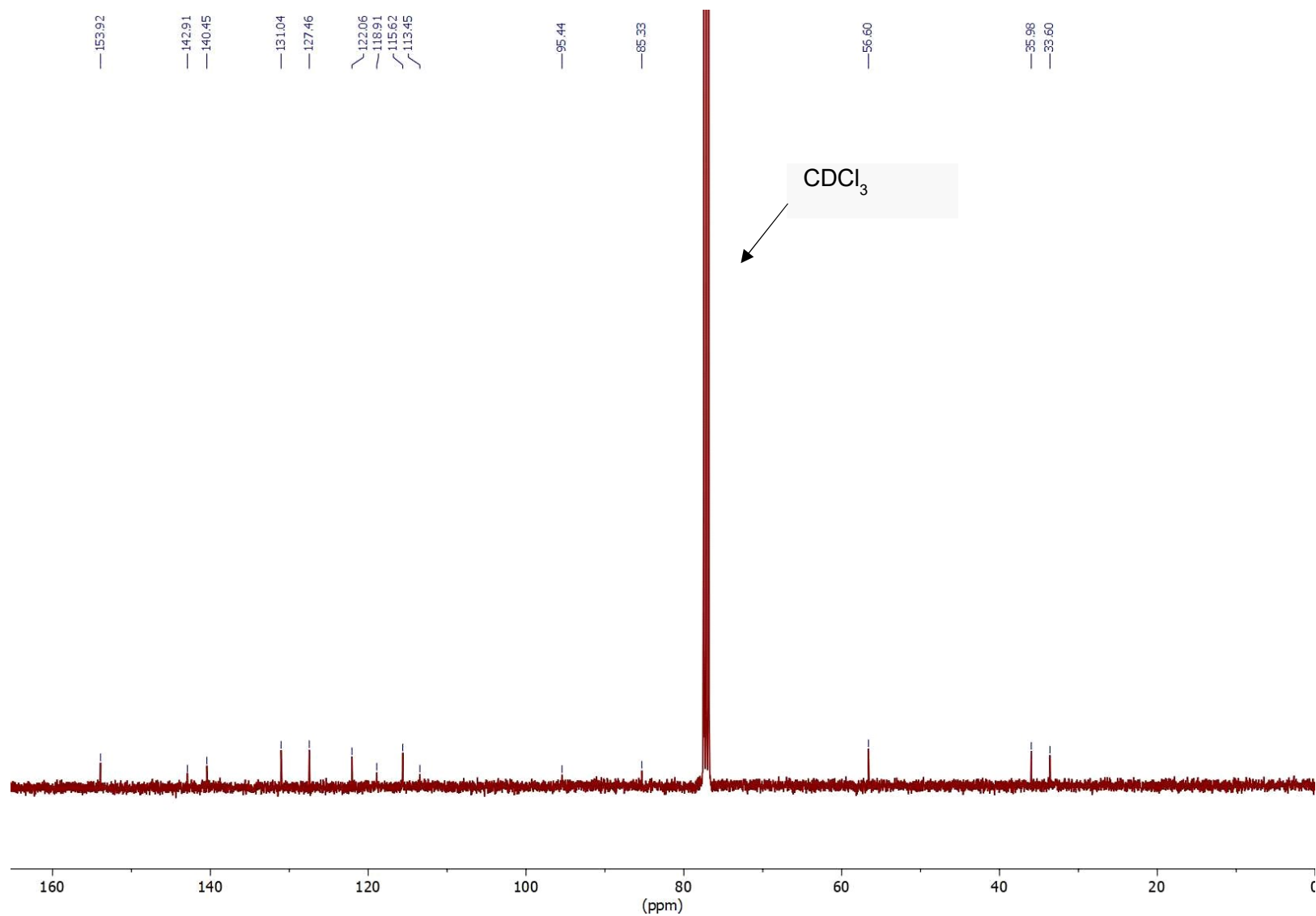
Figure 5. ^{13}\text{C} NMR spectrum of OPE3-Ph(OMe) 2 (125 MHz, \text{CDCl}_3 at 25 °C).
