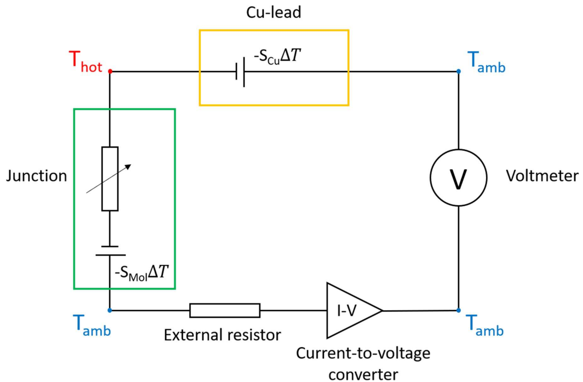
Figure 17. Electrical circuit and equivalent thermal circuit when V_{\text{bias}} is set to zero. The molecular junction (marked in green) is electrically equivalent to a conductance G and a thermovoltage (battery) in series. It is also necessary to include the thermovoltage that develops across the connecting copper lead (marked in yellow), due to the uncompensated temperature gradient.
