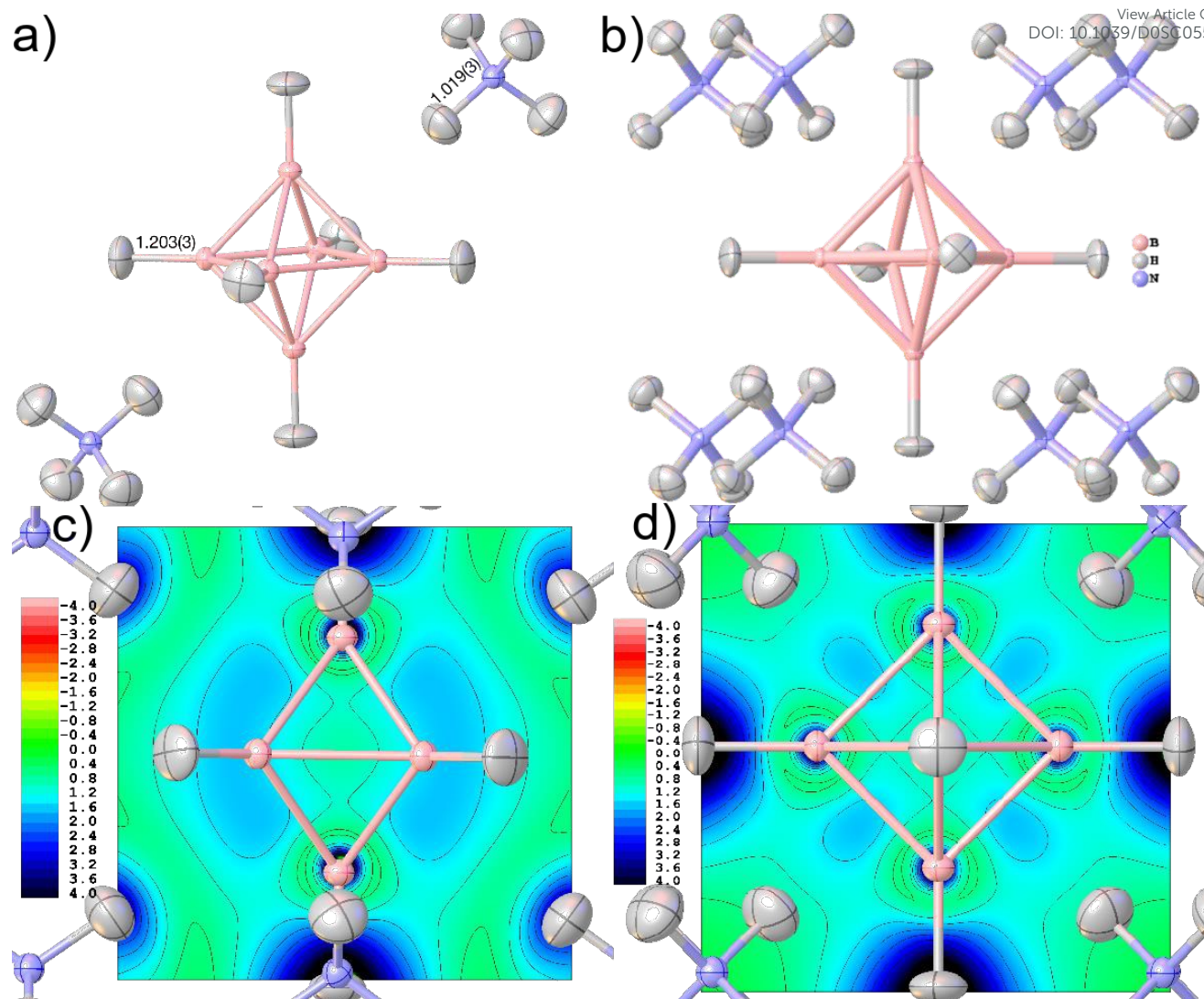
Figure 8. Final geometry and anisotropic displacement parameters at 80% probability level of ammonium borate (\text{NH}_4)_2\text{B}_6\text{H}_6 after HAR, showing (a) the formula unit with the two symmetry-independent refined bond distances in Å, and (b) the molecular cluster used in the wavefunction calculation. Electron localizability indicator ELI-D at contour intervals of 0.4 in a cut-plane (c) intersecting two pairs of opposite BBB faces, and (d) in the central boron square.
