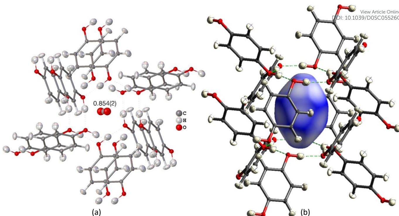
Figure 4. HAR-refined hydroquinone- \text{CO}_2 clathrate structure (HQ- \text{CO}_2 ) with anisotropic displacement parameters depicted at 80% probability level. The cluster of the guest \text{CO}_2 molecule with the 12 surrounding HQ molecules encapsulating \text{CO}_2 inside a void is shown as used in the wavefunction calculation underlying the non-spherical form factor generation. (a) Final refined geometry and partial occupation number of \text{CO}_2 . (b) Hirshfeld surface representation of \text{CO}_2 inside the void mapped with the property d_{\text{norm}} . Color scale from 0.08 (white) to 0.77 (blue). Generated with CrystalExplorer 87 .
