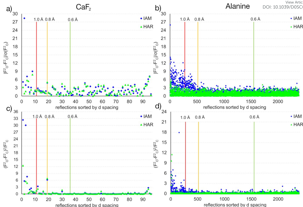
Figure 7. Differences of observed and calculated structure factors versus resolution for \text{CaF}_2 and L\text{-Ala} for the IAM and the HAR models.
