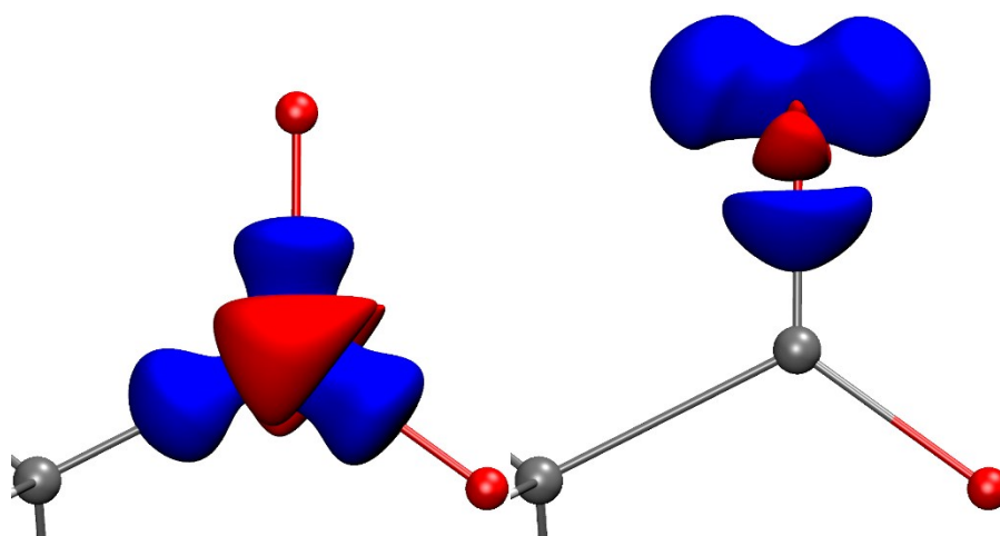
Figure 1. Deformation Hirshfeld densities 12 for the carbon (left) and oxygen (right) atoms in the carboxylate group of Gly-L-Ala, i.e. difference between the spherical atomic electron density used in the IAM and the non-spherical Hirshfeld atom density used in HAR (IAM minus HAR). Red = negative, blue = positive. Isovalue = 0.17 eÅ -3 .
