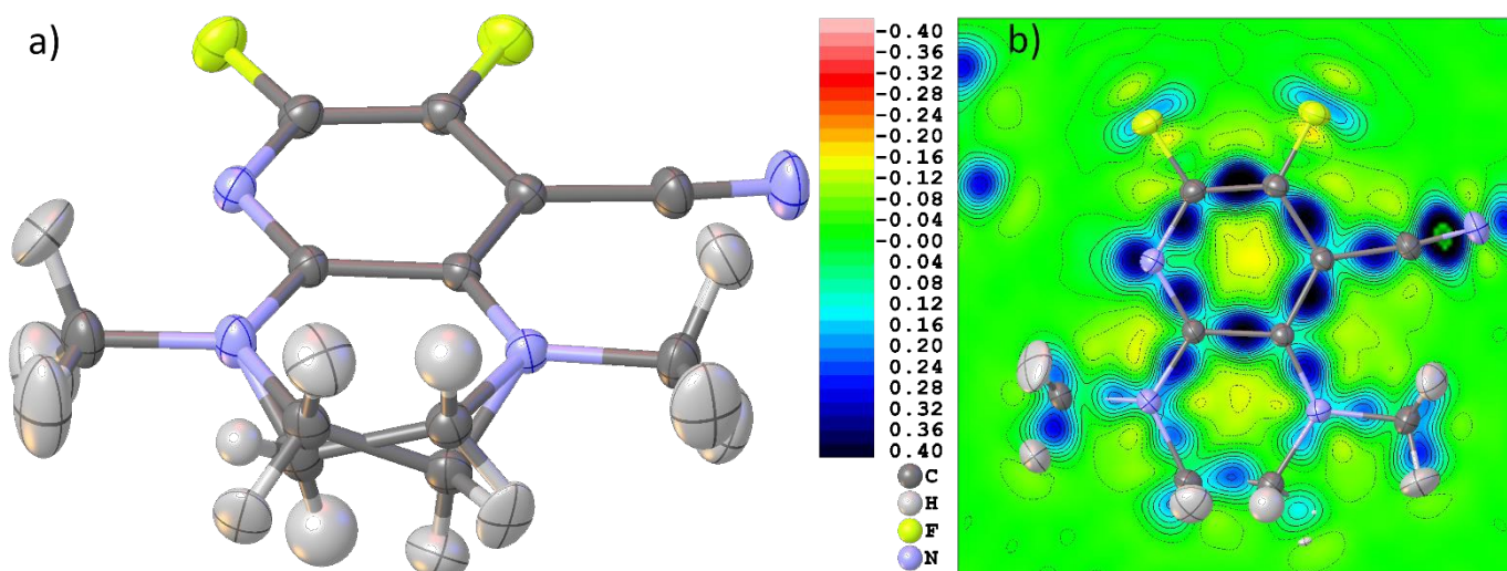
Figure 5. a) Final HAR geometry after disorder treatment of THPP. b) Dynamic deformation density distribution in the main molecular plane of the molecule. Color scale legend in \text{e\AA}^{-3} . Atomic anisotropic and isotropic displacement parameters at 80% probability level.
