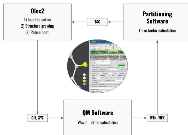
Figure 2. Flowchart of the process behind HAR controlled by NoSpherA2 and a visual representation of the GUI for NoSpherA2 inside Olex2 .
