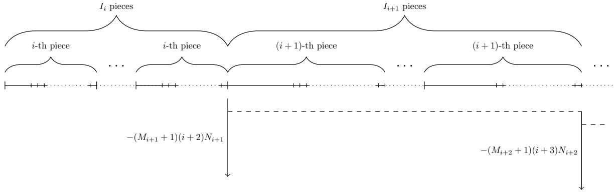
FIG 4. Picture of the bound encoded in (2.29). The downarrows represent the decrease at the end of the last i -th environment piece in comparison with the value at the beginning of the first i -th environment piece. The dashed line represents the upper bound on the supremum of the random walk.
