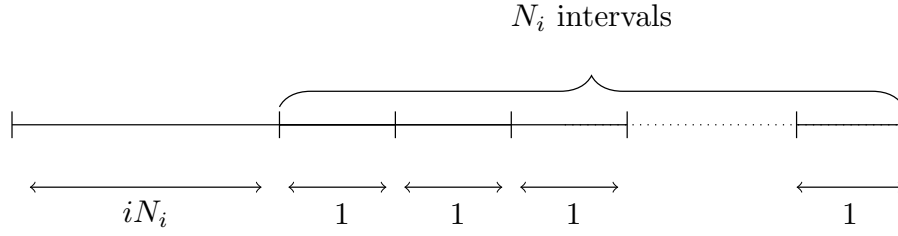
FIG 3. The i -th environment
