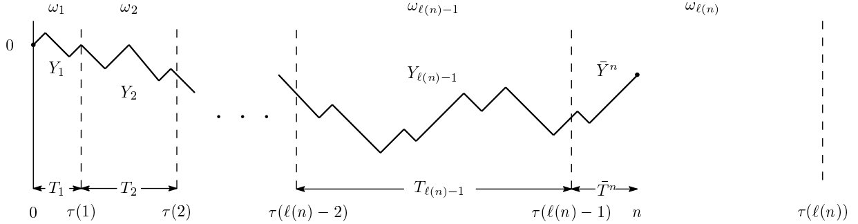
FIG 2. The decomposition of RWCRE into pieces of RWRE as in (1.14). The random variables (Y_k)_{1 \leq k < \ell(n)} ( Y_{\ell(n)} ) defined in (1.12) measure the spatial displacement (vertical axis) on each time interval [\tau(k) \wedge n, \tau(k+1) \wedge n] (horizontal axis).
