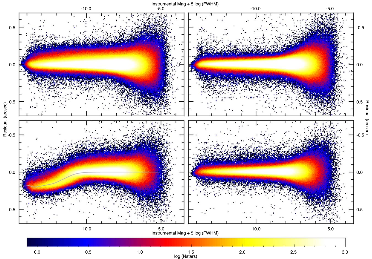
Figure 6. Illustration of the Koppenh fer effect on OTA04. Bottom left: X direction before correction. The solid line shows the measured mean residual for stars detected on this chip as a function of the instrumental magnitude/ \text{FWHM}^2 . Bottom right: Y direction before correction. Top left: X direction after correction. Top right: Y direction after correction.
