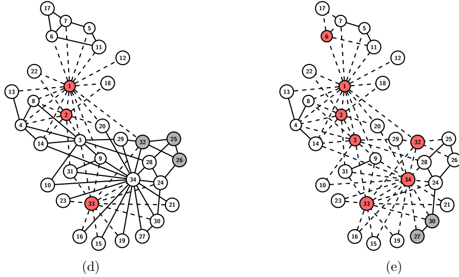
Figure 10: In part (d), we report an optimal CIP policy with k = 3 , depicting in red the interdicted vertices. In part (e), we report the same information for k = 7 .
