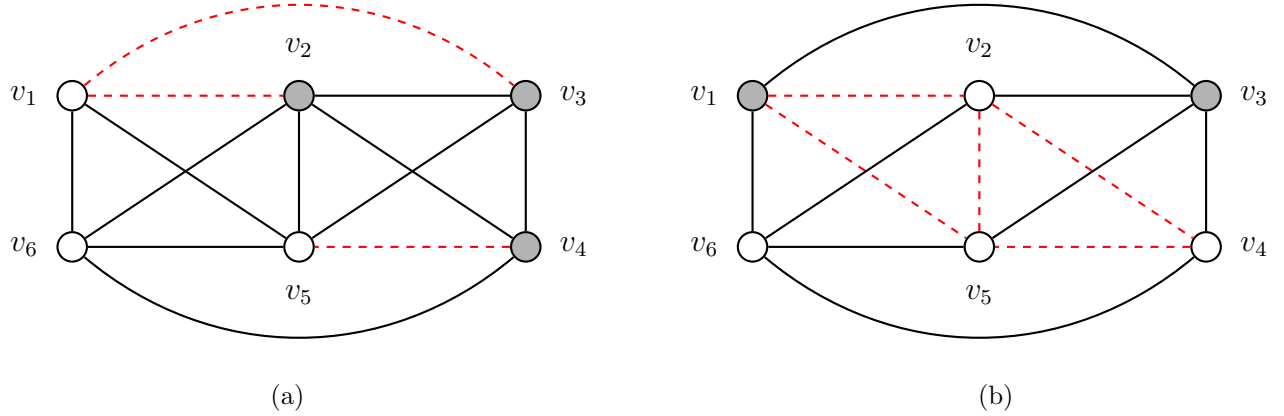
Figure 2: Two optimal interdiction policies represented by dashed red edges with: (a) k = 3 and (b) k = 5 . With k = 3 , the interdicted graph G_I has \omega(G_I) = 3 and one of the largest cliques is \{v_2, v_3, v_4\} (grey vertices). With k = 5 , \omega(G_I) = 2 and one of the largest cliques is \{v_1, v_3\} (grey vertices).
