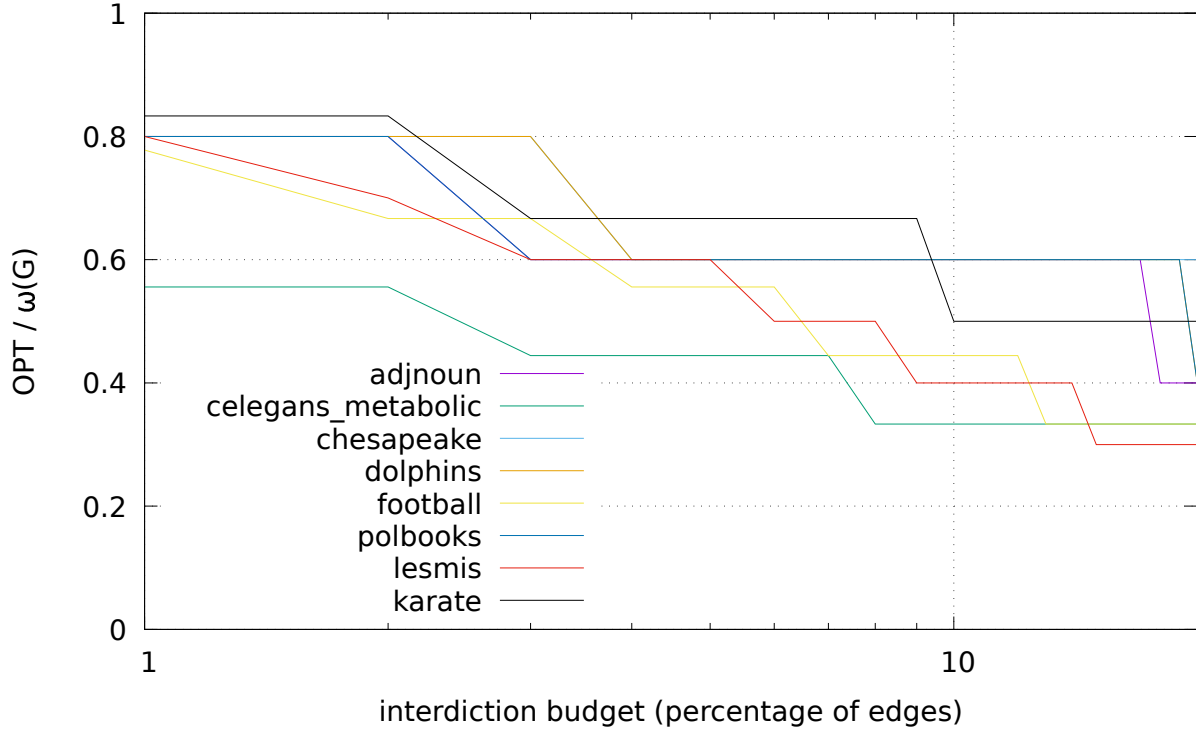
Figure 8: The edge clique interdiction curves for 8 classical (social) networks from the 10th DIMACS challenge [1].
