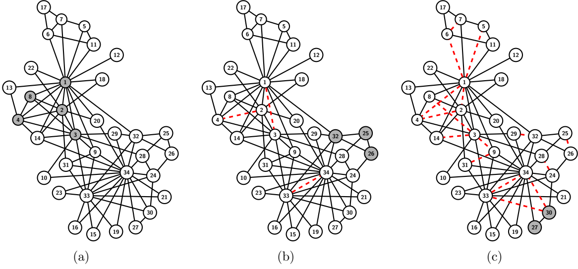
Figure 9: In part (a), we report the karate social network, grey vertices correspond to a maximum clique of size 5. In part (b), we report an optimal EICP policy with k = 3 , depicting in dashed red the interdicted edges. In this case, the size of the maximum clique in the interdicted graph is 3 and the grey vertices correspond to a maximum clique. In part (c), we report the same information for k = 16 .
