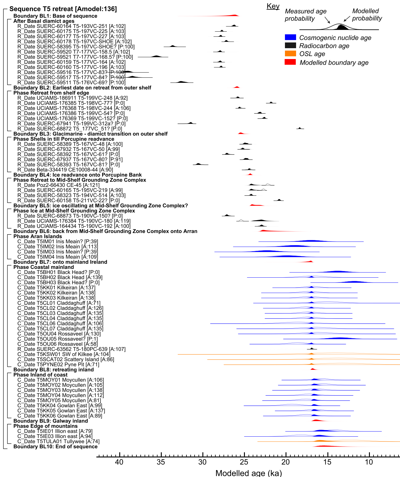
Figure 11. Bayesian age-model output for age measurements constraining the timing of ice sheet retreat in western Ireland and the adjoining continental shelf using OxCal (Bronk Ramsey, 2009). Agreement index (A-values in square brackets) shown alongside chronosequence conformability. P-values < 20 (in square brackets) denote outliers (underlined). Modelled age in ka cal BP on the x-axis. Each distribution (light grey) represents the relative probability of each age estimate with posterior density estimate (colour) generated by the modelling. Shown are ^{14}\text{C} ages (green), TCN ages (blue), OSL ages (orange) and modelled boundary ages (black). Each distribution represents the relative probability of each age estimate with posterior density estimate (coloured) generated by the modelling. [Color figure can be viewed at wileyonlinelibrary.com ]
