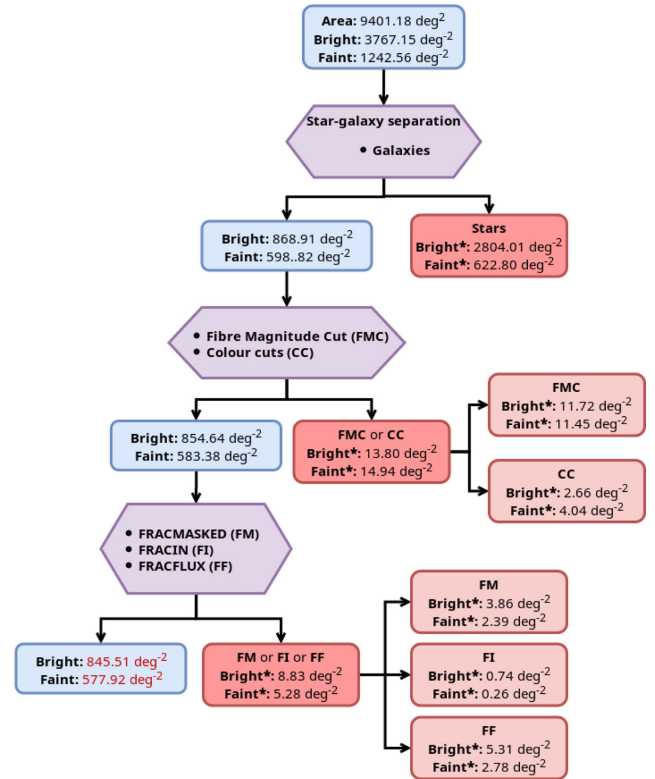
Figure 4. Flow chart of the BGS target selection in the Legacy Surveys DR8 based on photometric considerations. The photometric selection of BGS targets is divided into four stages: star–galaxy separation; fibre magnitude cuts (FMC); colour cuts (CCs); and quality cuts (QCs). The photometric cut flow chart is a continuation of the spatial cut flow chart (Fig. 2) and therefore we start from the area and object densities reported at the end of the spatial cut flow chart. We report densities for the bright and faint samples separately, showing in blue boxes the values for the sources remaining after each of the BGS cuts. The densities of the removed objects are shown in red/pink boxes. The different cuts applied are shown in purple hexagonal boxes.
