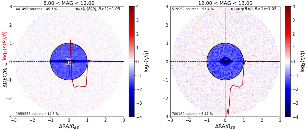
Figure 3. 2D histograms of the positions of BGS objects relative to their nearest Bright Star (BS) taken from the Gaia and Tycho-2 sources down to G -mag and visual magnitude MAG_{VT} of 13, respectively. These stacks are performed in magnitude bins in the BS catalogue from magnitude 8 to 12 (left) and from 12 to 13 (right). The stacks are made using angular separations rescaled to the masking radius function given in equation (3), which means that objects within a scaled radius of 0 to 1 will be masked out by the BS veto while objects with R = r/R_{BS} > 1 will not (here r^2 = (\Delta RA)^2 \cos^2(\text{Dec}) + \Delta \text{Dec}^2 ). The colour scale shows the ratio of the density per pixel ( \eta ) to the mean density ( \bar{\eta} ) within the shell 1.1 < r/R_{BS} < 3 . The density ratio is shown on a \log_2 scale where red shows overdensities, blue corresponds to underdensities, and white shows the mean density. The black solid circle shows extent of the BS exclusion zone. The red solid line shows the radial density profile on the same scale as the colour distribution \log_2(\eta(R)/\bar{\eta}) , where \eta(R) is the target density within the annulus at radius R of width \Delta R \sim 0.06 .
