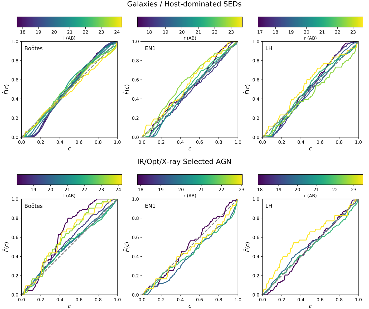
Fig. 10. Cumulative distribution of threshold credible intervals, c , ( \hat{F}(c) ) plot for the final consensus photo- z estimates for the galaxy (or host-dominated AGN) population ( top ) and the optical, infrared and X-ray selected AGN population ( bottom ) within each of the deep fields. Coloured lines represent the distributions in bins of apparent optical magnitude ( I -band for Boötes, r -band for EN1 and LH). Lines that fall above the 1:1 relation illustrate under-confidence in the photo- z uncertainties (uncertainties overestimated) while lines under illustrate over-confidence (uncertainties underestimated).
