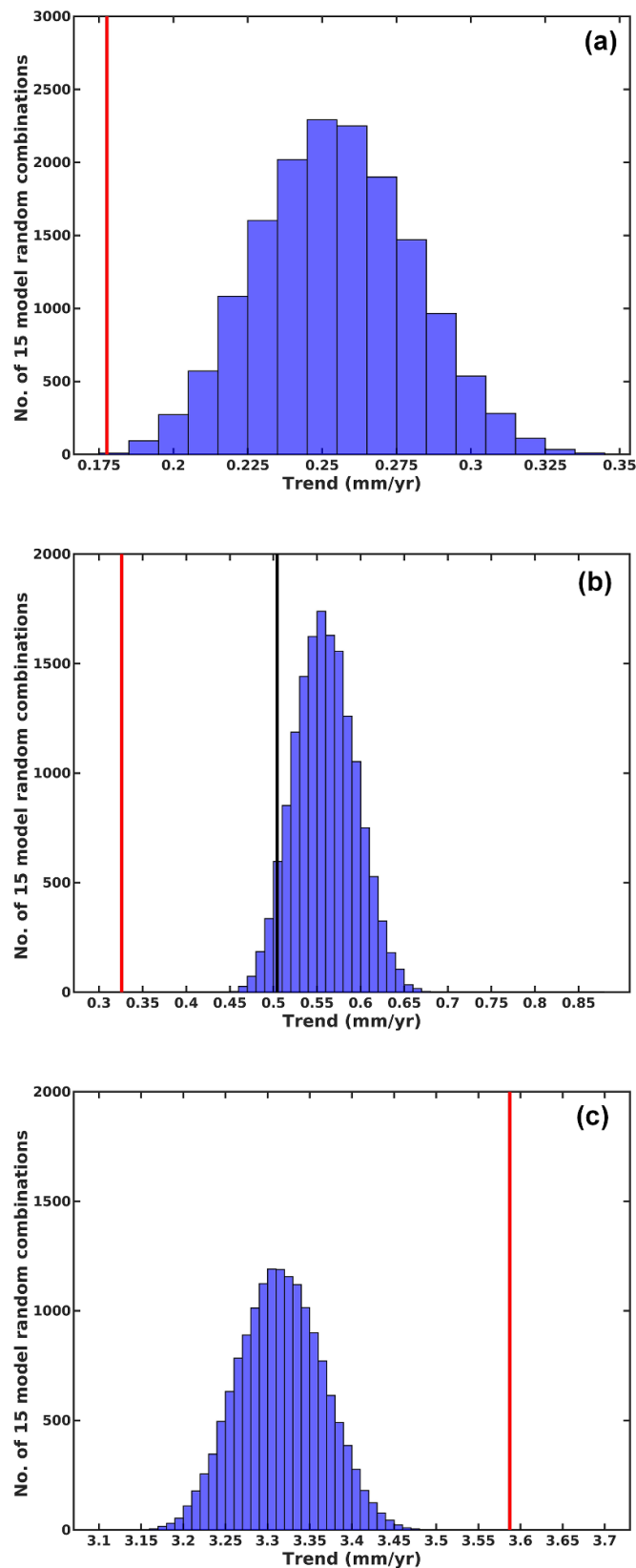
Figure 2. Histogram of CMIP5 MEM GMTSL trends (blue) from all combinations of 15 from 20 models compared to CMIP6 MEM GMTSL trend (red vertical line) over (a) historical period 1901–1990, (b) observational period 1957–2005 and (c) future RCP8.5/SSP585 projections over 2015–2100. Black vertical line (panel b) indicates GMTSL trend from observations (0–2000 m), compare to the model simulations for the full ocean depth.
