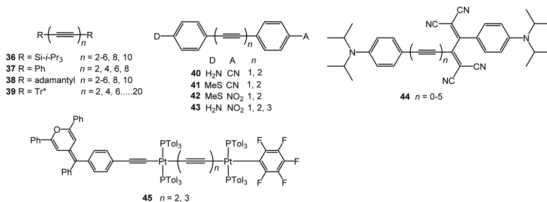
Fig. 15 Structures of 36–45 .
