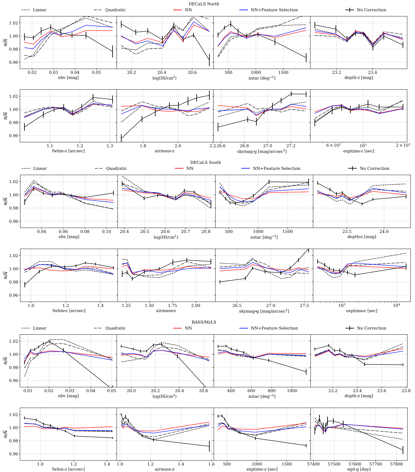
Figure 8. Target density variation of the photometric sample with imaging systematics before applying weights (black) and after assuming a linear (dotted), quadratic (dashed) or NN based (red) relation between the observed galaxy density and the potential systematics. The blue curves show the correction based on NN and after applying a feature selection that avoids overfitting and is described in Appendix A. Top: DECaLS-North, middle: DECaLS-South, and bottom: BASS/MzLS.
