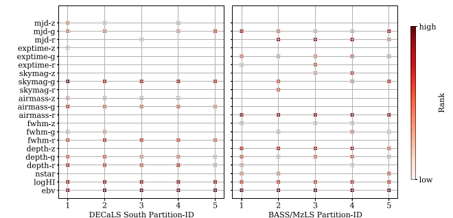
Figure A1. Important imaging maps according to the feature selection procedure for DECaLS-South (left) and BASS/MzLS (right). The selected maps are shown with circles and their rank is colour coded to represent the more important maps with the darker circles.
