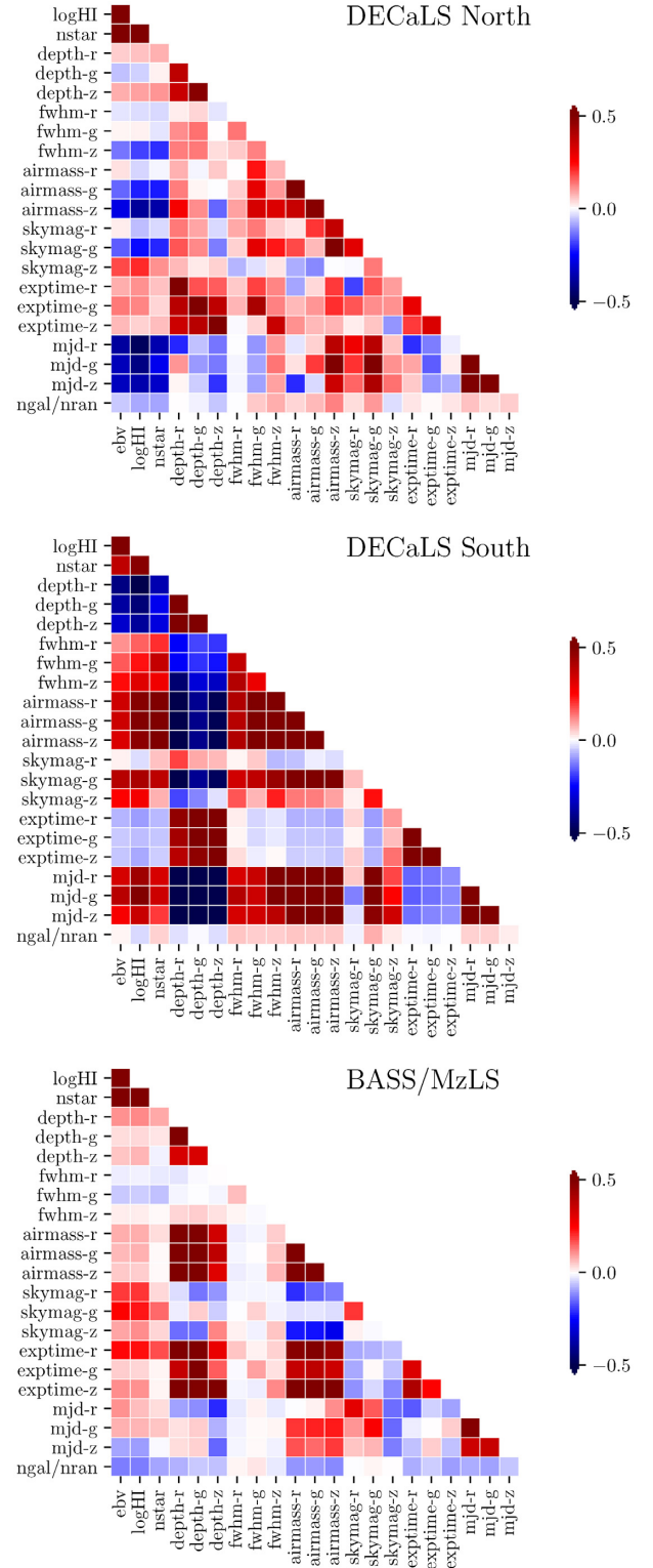
Figure 7. Correlation coefficients between each imaging systematics and the observed galaxy density. Top: DECaLS-North, middle: DECaLS-South, and bottom: BASS/MzLS.
