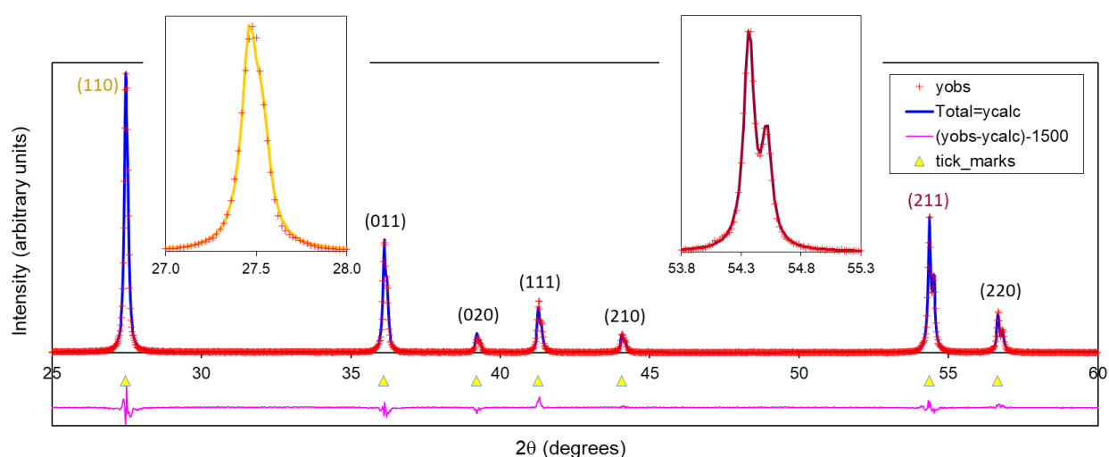
Figure 6. Rietveld fit to experimental data discussed in Section 7. Observed data shown as red crosses, calculated as a solid blue line and the difference curve (offset) as a pink line. Arrows show the predicted 2\theta values of different hkl reflections. Insets show zooms of the (110) and (211) reflections. Note how the K_{\alpha 1/\alpha 2} radiation leads to clear peak splitting at higher 2\theta .
