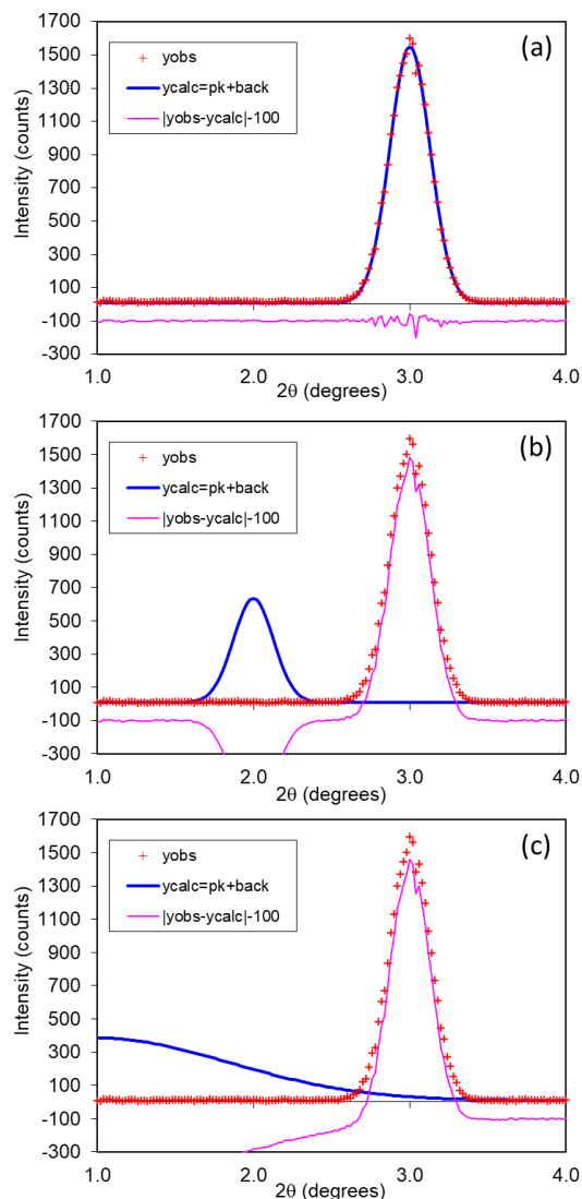
Figure 4. Fitting a Gaussian function in Excel. (a) shows the converged fit. (b) shows ( pos, int, fwhm = 2.0, 200, 0.3 ), which does not converge. (c) shows ( pos, int, fwhm = 1.0, 800, 2.0 ), which does converge.
