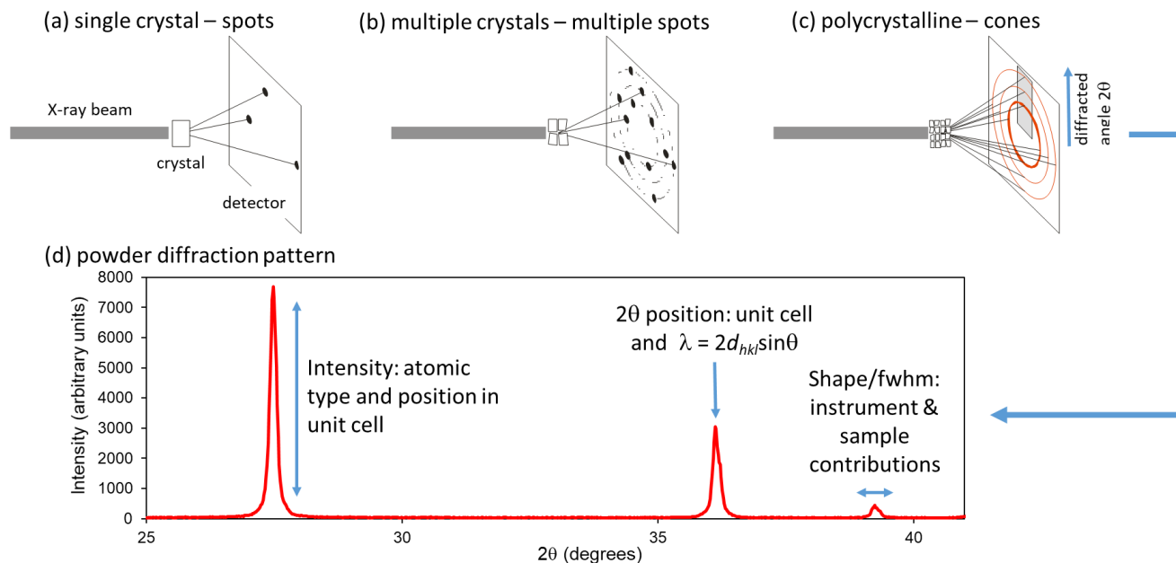
Figure 2. A single crystal gives rise to diffracted beams in discrete directions which appear as "spots" on a 2D detector. With multiple crystals, spots will be seen from each crystal. In a powdered or polycrystalline sample this leads to cones of diffracted intensity which are intersected as circles on a 2D detector, each circle corresponds to an individual or overlapped set of hkl reflections. A one-dimensional scan in 2\theta across these rings (or integration around them) leads to (d) a powder diffraction pattern as a plot of diffracted intensity as a function of angle 2\theta .
