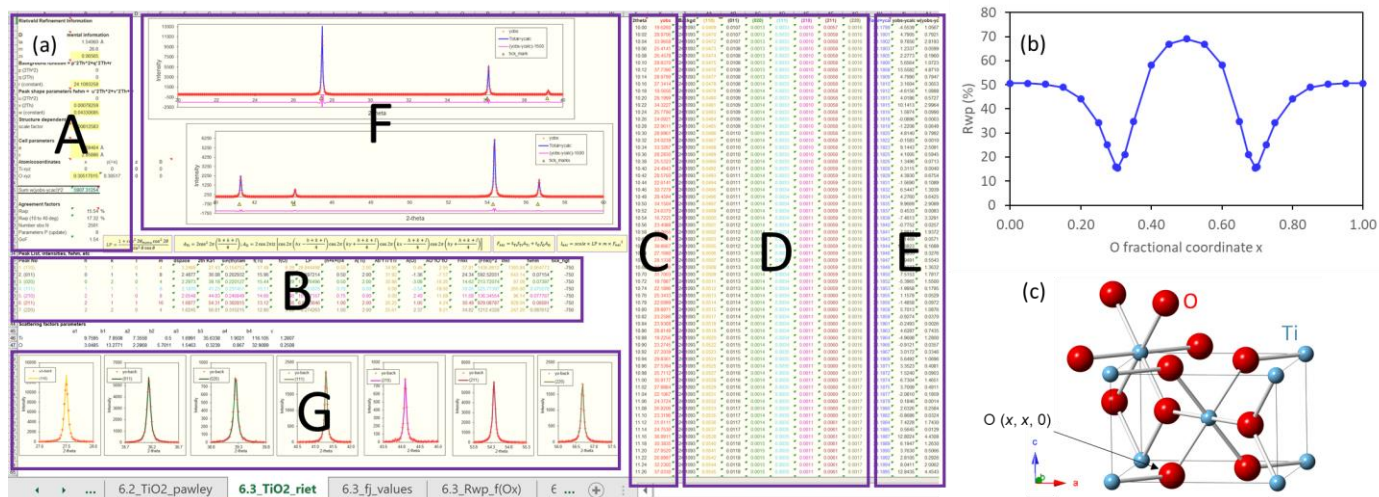
345 Figure 5. (a) Excel spreadsheet used for Rietveld refinement, with annotated sections discussed in the text. (b) Dependence of R_{wp} on fractional atomic coordinate x of O on site (x, x, 0) . (c) The rutile structure (Ti blue, oxygen red); oxygen sites in neighboring unit cells are included to show the coordination sphere around a Ti on one cell corner.
