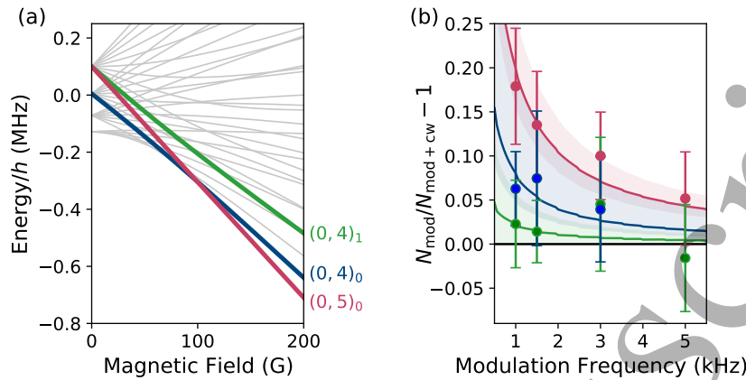
Figure 2. (a) Hyperfine Zeeman structure of RbCs in the rovibrational ground state. The states used in this work are highlighted in bold colours and labelled by (n, m_{f, \text{RbCs}})_k as defined in the main text. (b) Fractional change in the molecule number N_{\text{mod}}/N_{\text{mod}+\text{CW}} - 1 as a function of the modulation frequency of the trap light intensity. Results are shown for molecules in (0, 5)_0 in red, (0, 4)_0 in blue, and (0, 4)_1 in green, with all measurements performed at a magnetic field of 181.6 G. We observe a smaller suppression of the collisional loss for molecules not occupying the hyperfine ground state (0, 5)_0 . The lines show fits to the results using the numerical model in Eq. 2 for \Phi = 1 , with the 1\sigma uncertainty in the lifetime of the complex in the dark indicated by the shaded regions for each fit.
