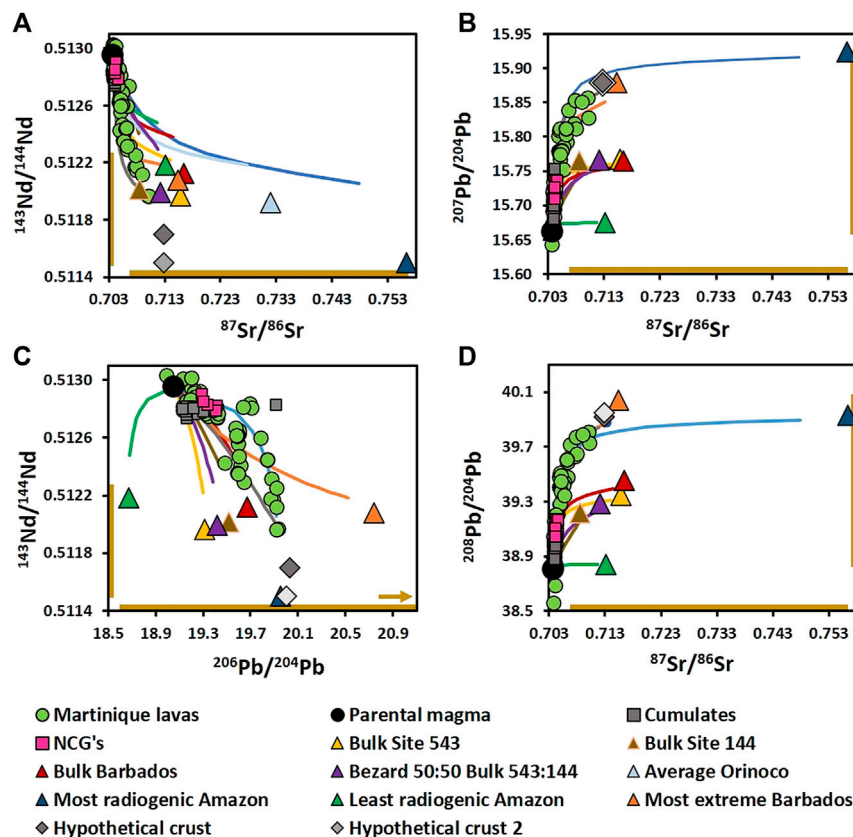
FIGURE 10 | (A) ^{87}\text{Sr}/^{86}\text{Sr} vs. ^{143}\text{Nd}/^{144}\text{Nd} , (B) ^{87}\text{Sr}/^{86}\text{Sr} vs. ^{207}\text{Pb}/^{204}\text{Pb} , (C) ^{206}\text{Pb}/^{204}\text{Pb} vs. ^{143}\text{Nd}/^{144}\text{Nd} and (D) ^{87}\text{Sr}/^{86}\text{Sr} vs. ^{208}\text{Pb}/^{204}\text{Pb} , for Martinique lavas, plutonic xenoliths (this study) and end members used in AFC modeling from Table 3. Data sources as per Table 3 and Figure 8. For all data points, uncertainty (2 SE) is smaller than symbol size. Brown bars along axes show range of isotopic compositions of sediments potentially equivalent to those in the arc crust from Figure 8. Colored curves correspond to AFC models for each crustal end member, shown in detail in Figure 11.
