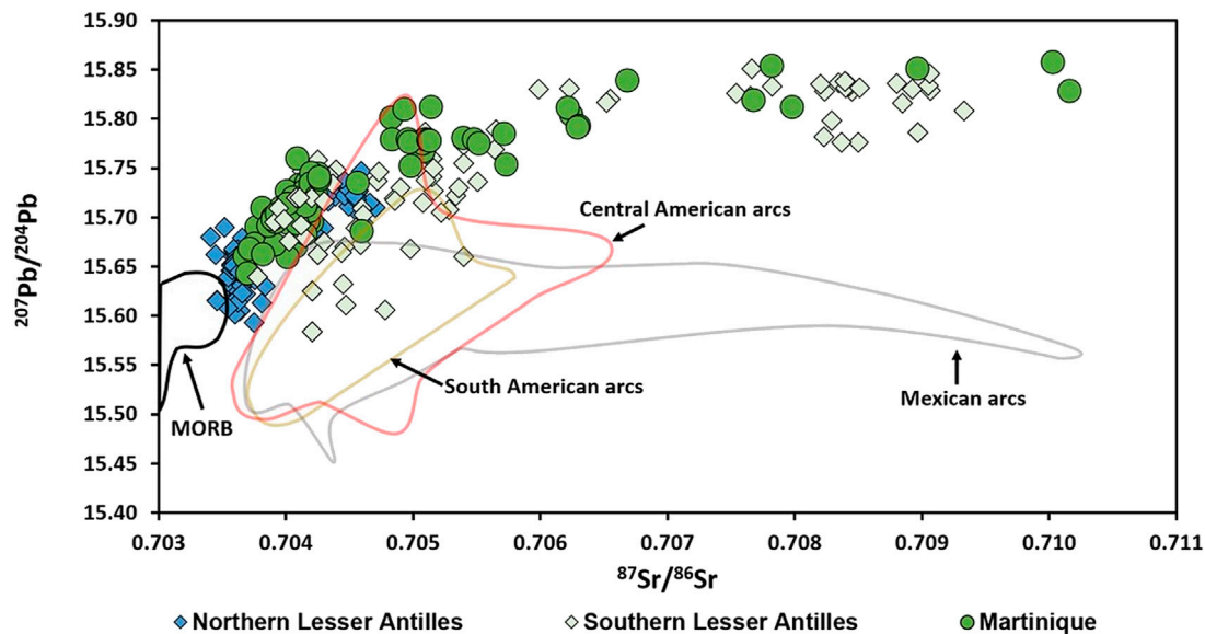
FIGURE 2 | ^{87}\text{Sr}/^{86}\text{Sr} vs. ^{207}\text{Pb}/^{204}\text{Pb} of lavas from the Lesser Antilles arc, compared to nearby arcs from Central-South America shown in Figure 1 . For all data points, uncertainty (2 SE) is smaller than symbol size. Northern Lesser Antilles = Saba to Dominica. Southern Lesser Antilles = Martinique to Grenada (Martinique data shown separately). Data sources: Northern Lesser Antilles—Van Soest et al. (2002); Lindsay et al. (2005); Toothill et al. (2007); DuFrane et al. (2009); Davidson and Wilson (2011). Southern Lesser Antilles—Thirlwall and Graham (1984); Davidson (1986); White and Dupre (1986); Smith et al. (1996); Thirlwall et al. (1996); Turner et al. (1996); Heath et al. (1998); Labanieh et al. (2010); Huang et al. (2011); Bezard et al. (2014). Southern American, Central American and Mexican arc data from the Georoc database ( http://georoc.mpch-mainz.gwdg.de/georoc/ ). MORB data from the PetDB database ( www.earthchem.org/petdb ) for Mid-Atlantic Ridge basalts 30^\circ either side of the equator. Labanieh et al. (2010) found that the difference between measured and age corrected isotope ratios for the oldest lavas in the arc ( \sim 25 Ma, from Martinique) was negligible. Since majority of lavas in the LAA are much younger than 25 Ma, age correction is considered negligible by majority of authors and would not alter the trend shown.
