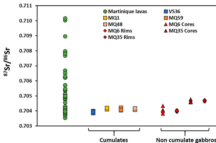
FIGURE 5 | ^{87}\text{Sr}/^{86}\text{Sr} of individual plagioclase in cumulates, and core and rim zones of plagioclase in NCG's, compared with the whole rock ^{87}\text{Sr}/^{86}\text{Sr} range of Martinique lavas. Lava data from Davidson (1986) and Labanieh et al. (2010). For all data points, uncertainty (2 SE) is smaller than symbol size.
