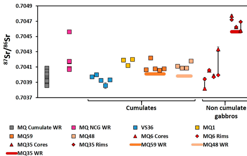
FIGURE 6 | Details of ^{87}\text{Sr}/^{86}\text{Sr} variation in cumulate and NCG plagioclase. The whole rock ^{87}\text{Sr}/^{86}\text{Sr} range for Martinique cumulates and NCG's is plotted for comparison. Whole rock data for individual samples shown as colored bars (bar width covers uncertainty). Where visible, black bars show uncertainty (2 SE), otherwise uncertainty is smaller than symbol size. Core-rim pairs are joined by tie lines.
