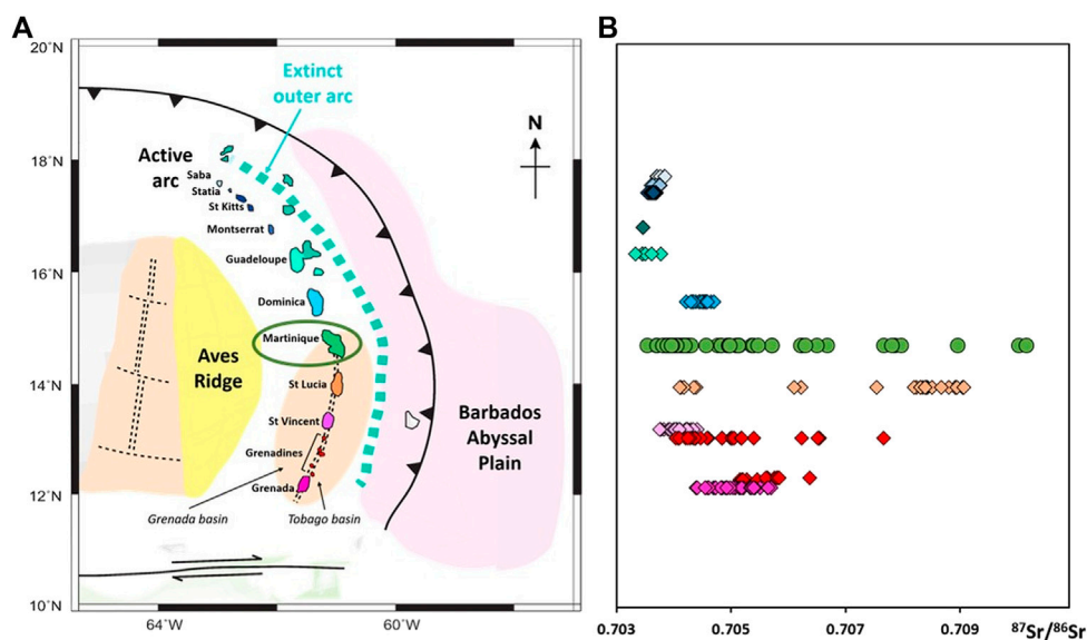
FIGURE 3 | (A) Map of Lesser Antilles arc (region marked by black outlined box on Figure 1 ) modified from Allen et al. (2019). (B) Compilation of along arc variation in ^{87}\text{Sr}/^{86}\text{Sr} of lavas. For all data points, uncertainty (2 SE) is smaller than symbol size. Data sources are the same as Figure 2 . Note that the same along arc trends are also observed in the Nd and Pb isotopic systems.
