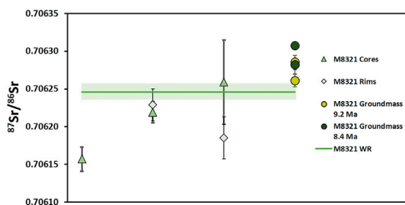
FIGURE 7 | Details of ^{87}\text{Sr}/^{86}\text{Sr} variation in lava sample M8321. The whole rock value from Davidson (1986) is plotted for comparison. Black and gray bars (and green box around the WR value) show uncertainty (2 SE).
