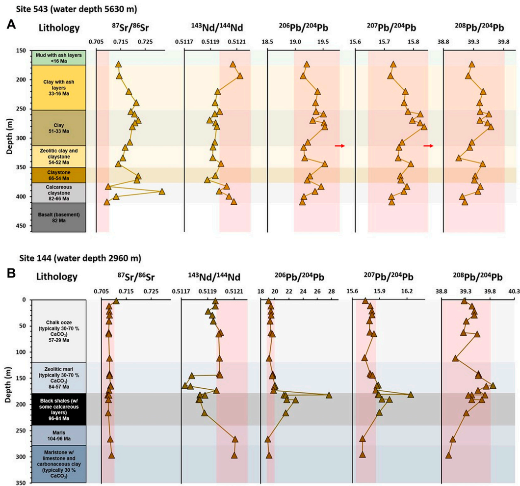
FIGURE 9 | (A): Radiogenic isotopic compositions of DSDP Site 543 sediments, modified from Carpentier et al. (2008). (B): Radiogenic isotopic compositions of DSDP Site 144 sediments, modified from Carpentier et al. (2008). Pink bar indicates isotopic range of Martinique lavas (data sources as per Figure 8). For all data points, uncertainty (2 SE) is smaller than symbol size. Red arrows in (A) indicate that range of lavas exceeds the scale shown on the plot.
