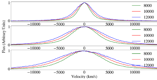
Figure 2. Modelled Ly \alpha emission spectra of the spherical BLR model as a function of the maximum standard deviation (8000, 10 000, and 12 000 km s -1 for the green, red, and blue curves, respectively) for different inner radius, r_{\min} = 0.01, 0.05, and 0.1, for the top to bottom panels, respectively.
